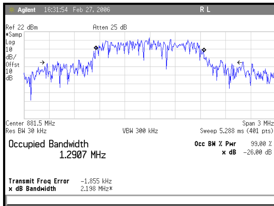
Plot 6. CDMA Downlink Output
