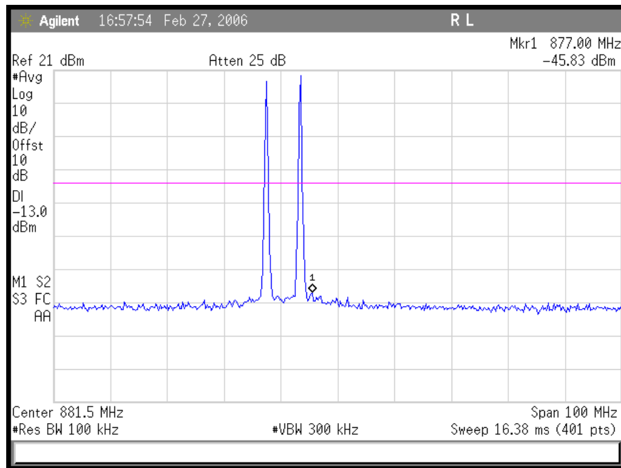
Plot 31. AMPS Down Link Low End Intermodulation
