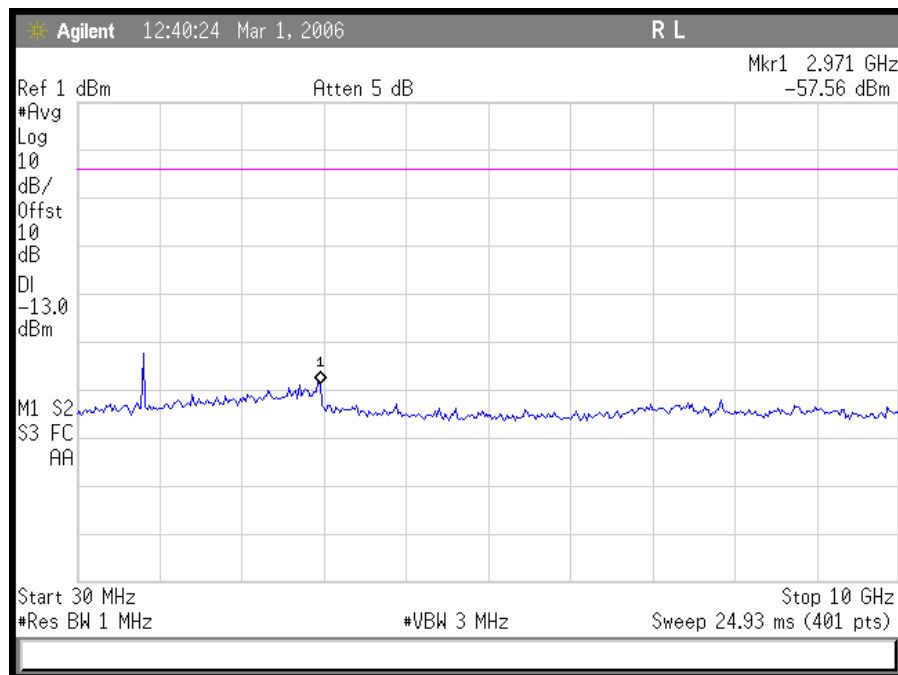
Plot 28. TDMA UpLink Low CH Conducted Emissions 30 MHz – 10 GHz
