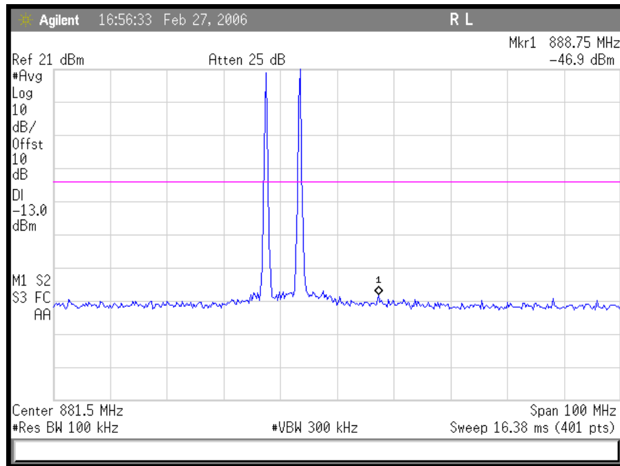
Plot 39. TDMA Down Link Low End Intermodulation
