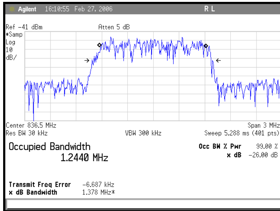
Plot 7. CDMA Uplink Input
