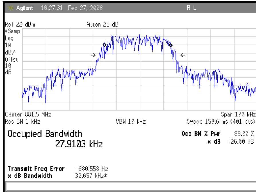
Plot 10. TDMA Downlink Output
