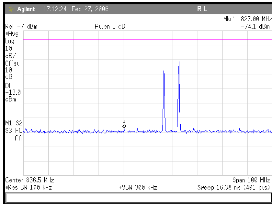
Plot 42. TDMA Uplink High End Intermodulation
