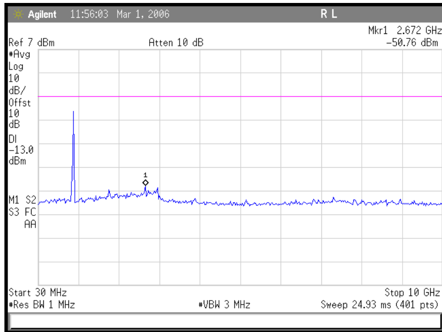
Plot 15. AMPS Downlink High CH Conducted Emissions 30 MHz – 10 GHz
