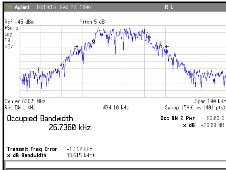
Plot 3. AMPS Uplink Input
