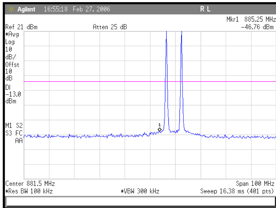
Plot 40. TDMA Down Link High End Intermodulation
