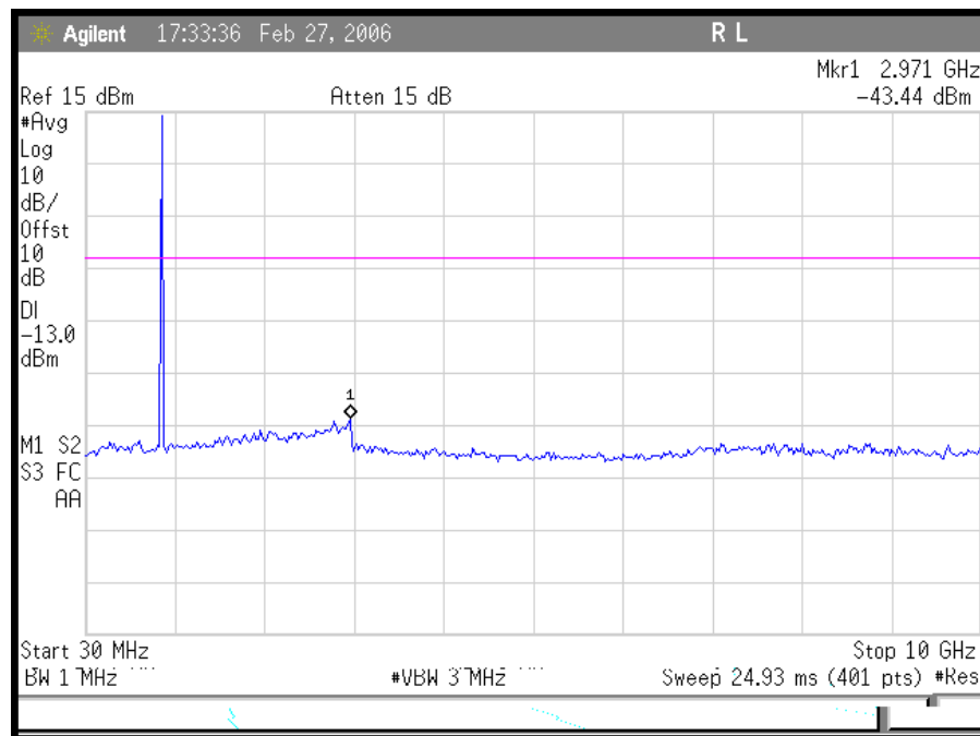
Plot 26. TDMA Downlink Mid CH Conducted Emissions 30 MHz – 10 GHz
