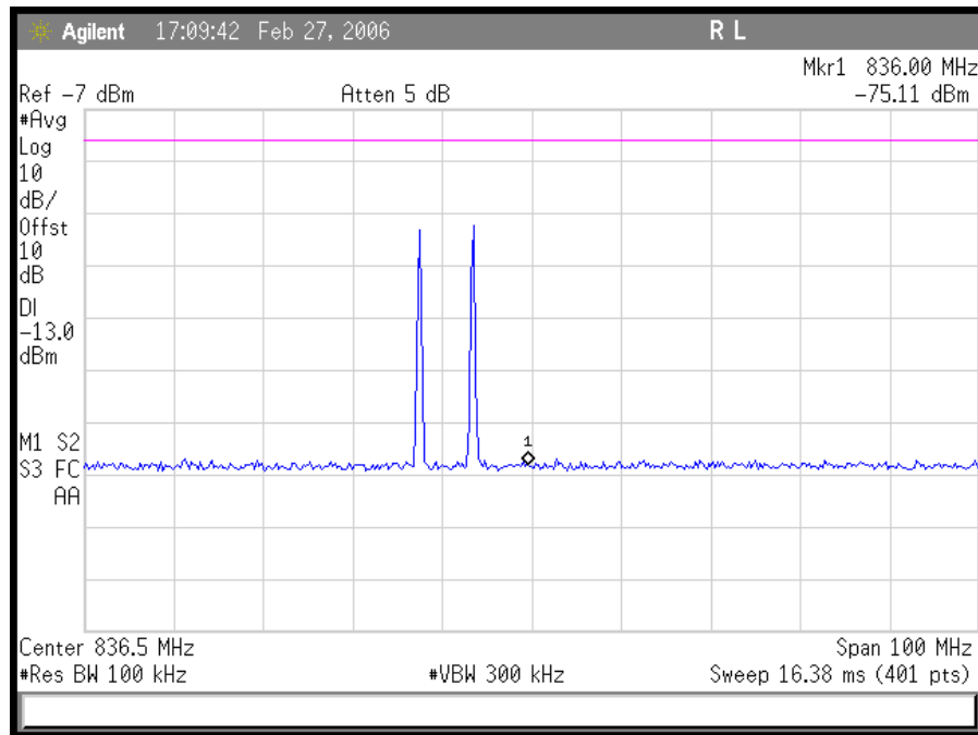
Plot 33. AMPS Uplink Low End Intermodulation
