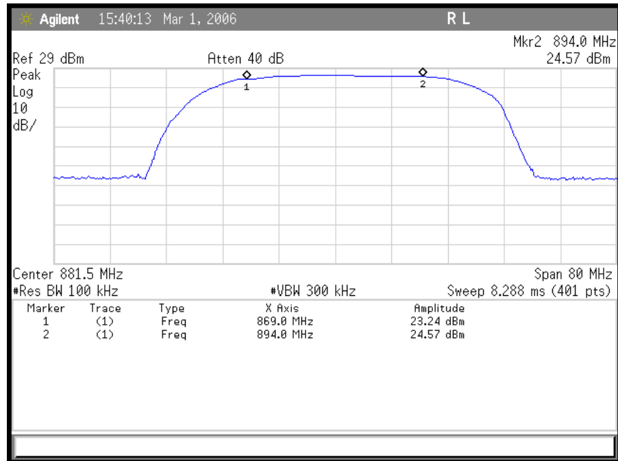
Plot 43. Part 22 Downlink Out of Band Rejection
