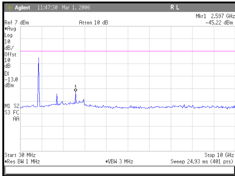
Plot 19. CDMA Downlink Low CH Conducted Emissions 30 MHz – 10 GHz
