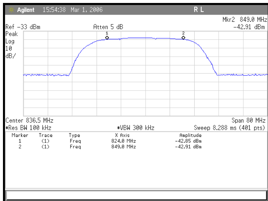
Plot 44. Part 22 Uplink Out of Band Rejection
