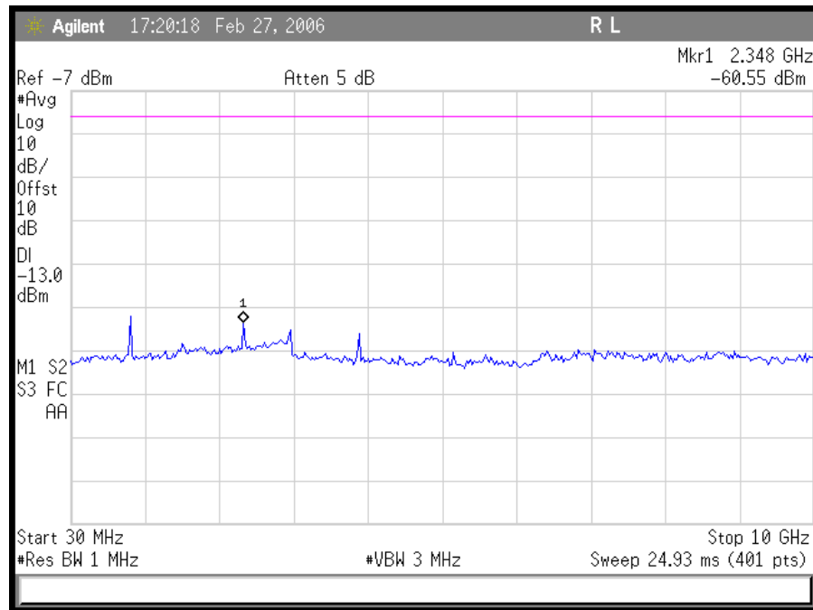
Plot 23. CDMA Uplink Mid CH Conducted Emissions 30 MHz – 10 GHz
