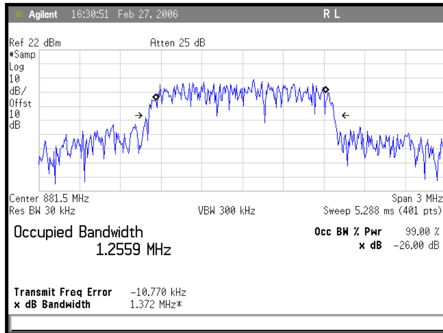
Plot 5. CDMA Downlink Input
