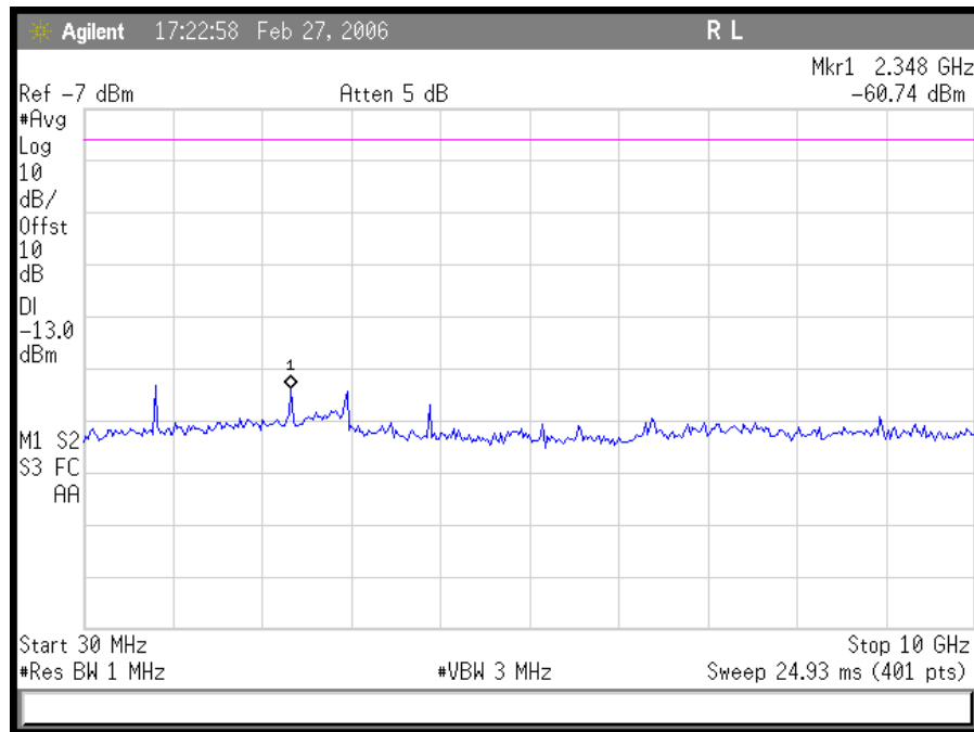
Plot 17. AMPS Uplink Mid CH Conducted Emissions 30 MHz – 10 GHz
