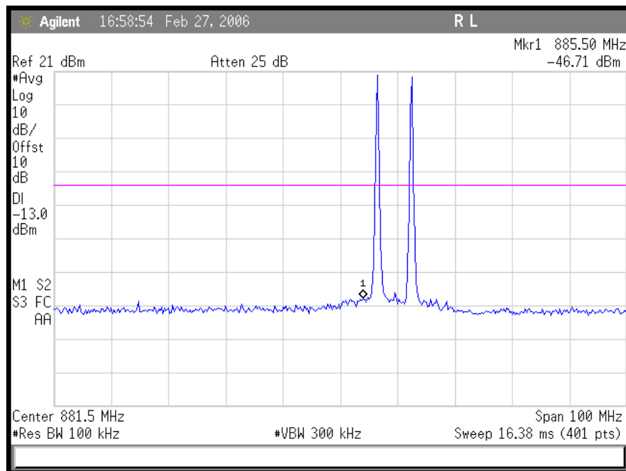
Plot 32. AMPS Down Link High End Intermodulation
