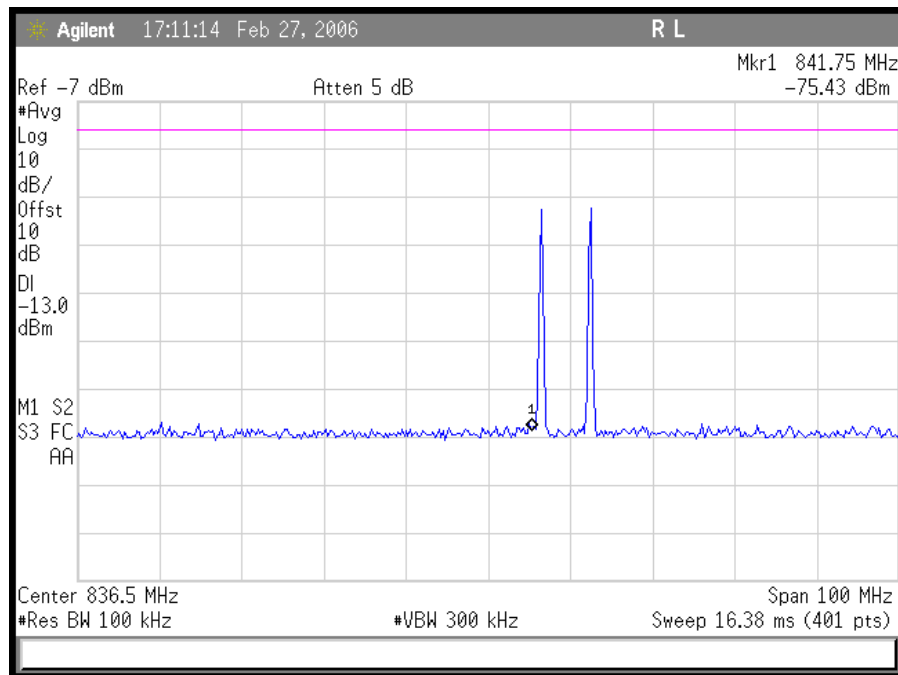
Plot 34. AMPS Uplink High End Intermodulation
