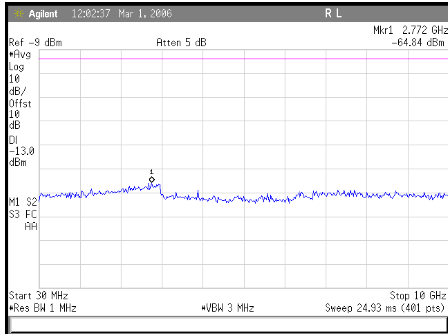
Plot 24. CDMA Uplink High CH Conducted Emissions 30 MHz – 10 GHz
