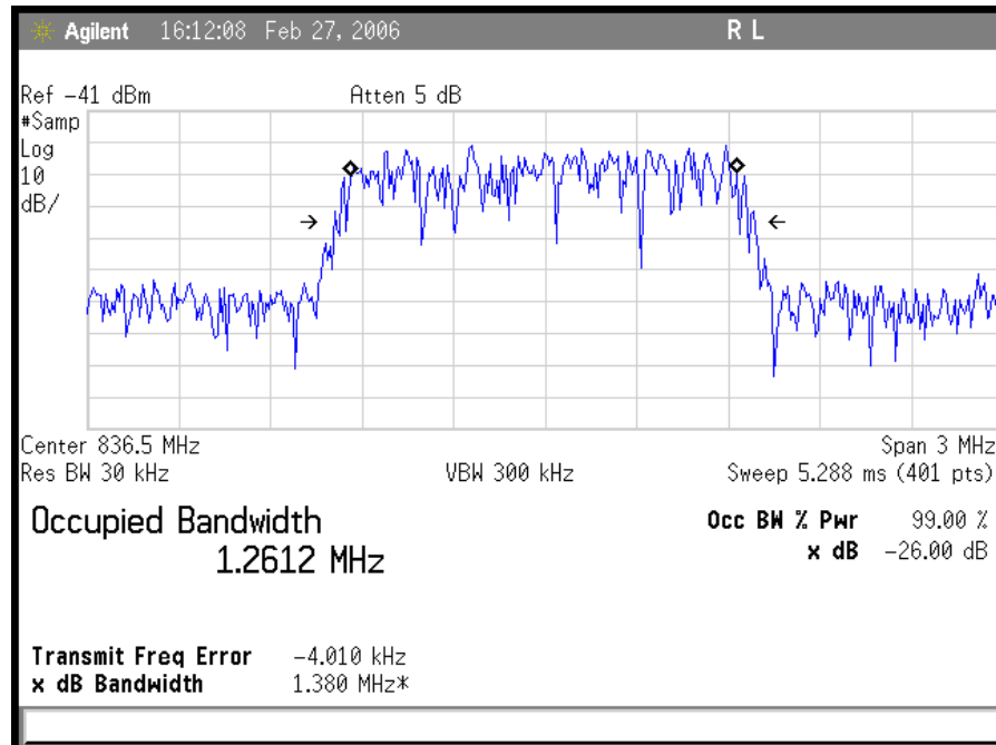
Plot 8. CDMA Uplink Output
