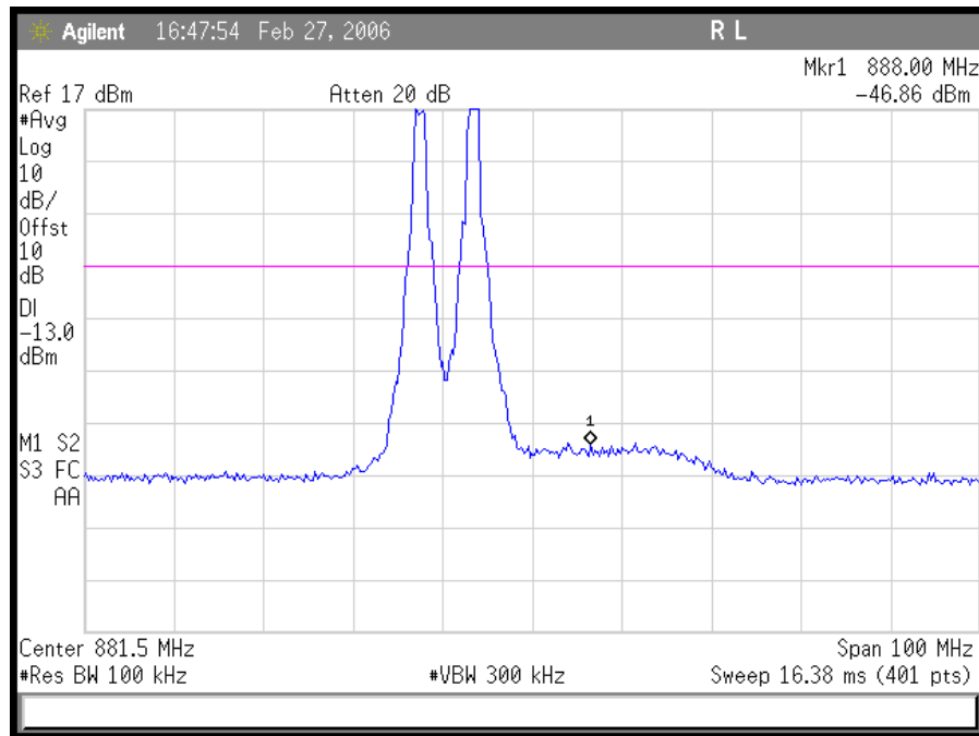
Plot 35. CDMA Down Link Low End Intermodulation
