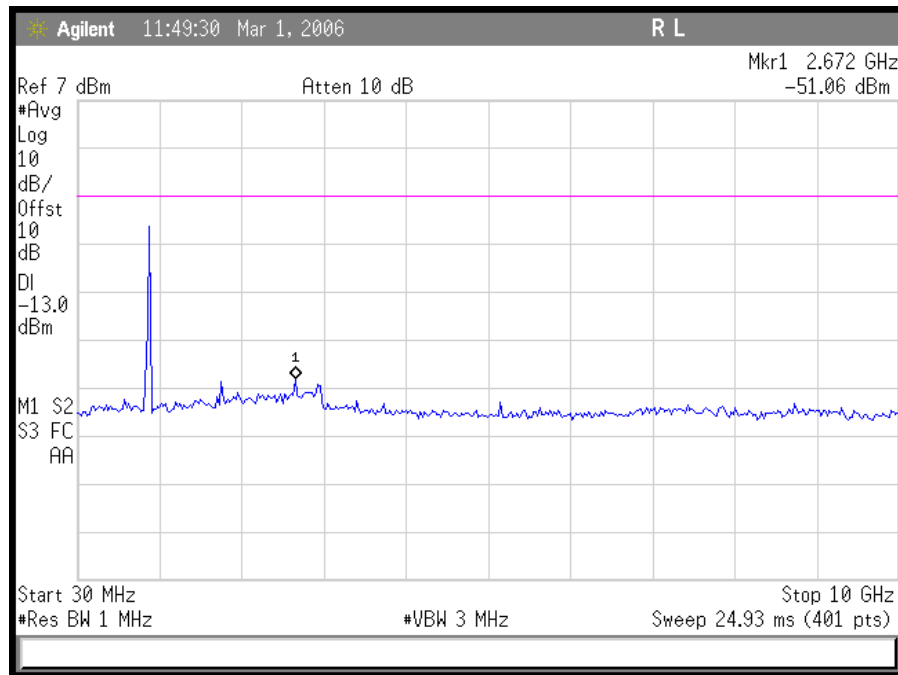
Plot 27. TDMA Downlink High CH Conducted Emissions 30 MHz – 10 GHz
