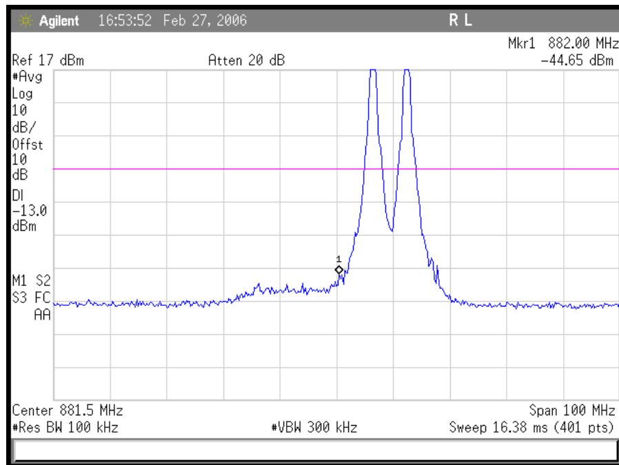
Plot 36. CDMA Down Link High End Intermodulation
