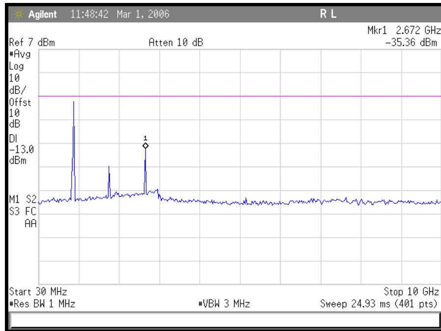
Plot 21. CDMA Downlink High CH Conducted Emissions 30 MHz – 10 GHz
