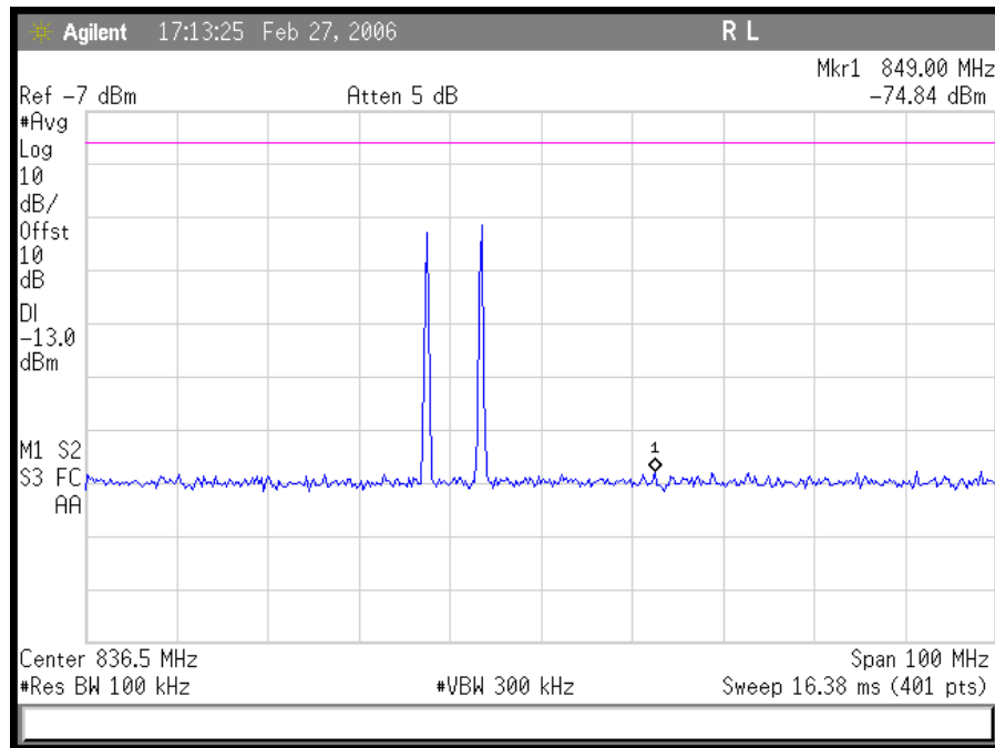
Plot 41. TDMA Uplink Low End Intermodulation
