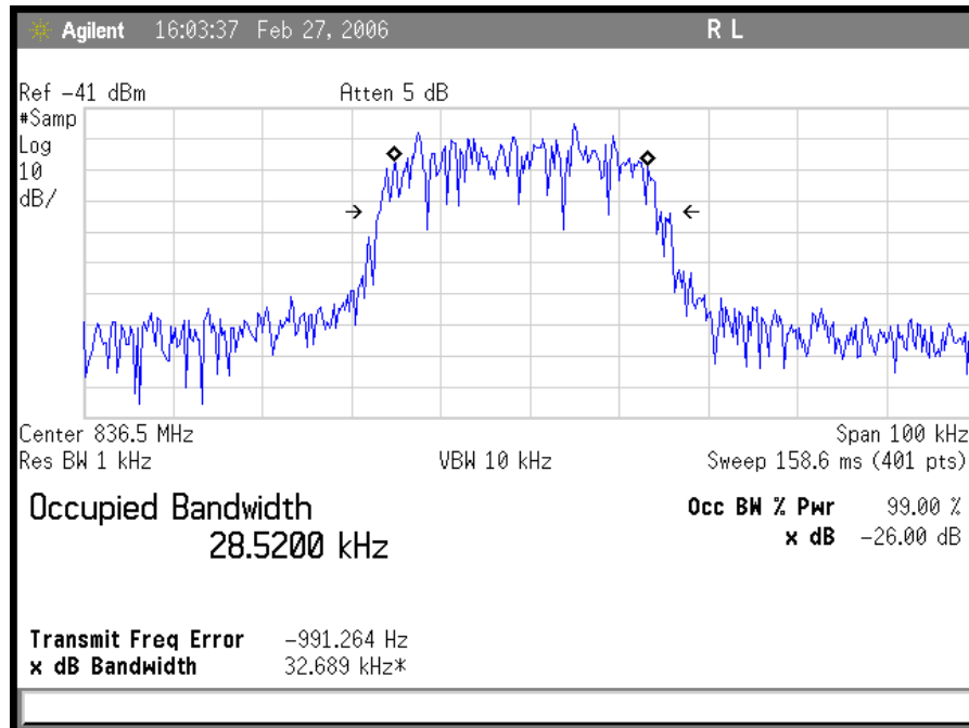
Plot 12. TDMA Uplink Output
