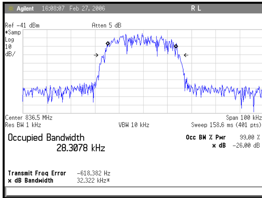
Plot 11. TDMA Uplink Input
