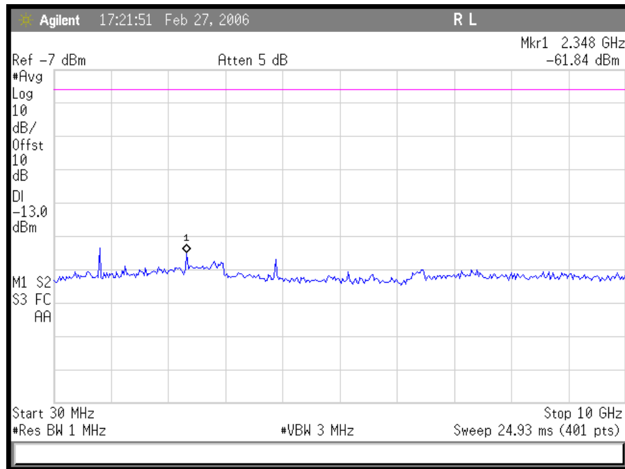
Plot 29. TDMA Uplink Mid CH Conducted Emissions 30 MHz – 10 GHz
