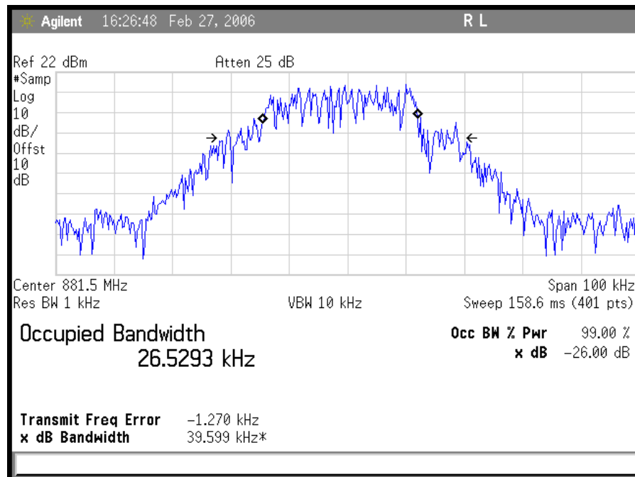
Plot 2. AMPS Downlink Output
