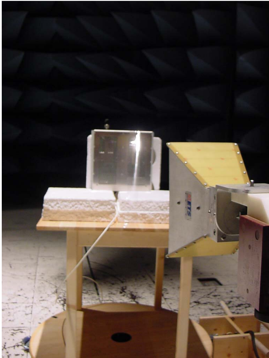
Photograph 2. Test Equipment and setup for Radiated Harmonic Measurements
