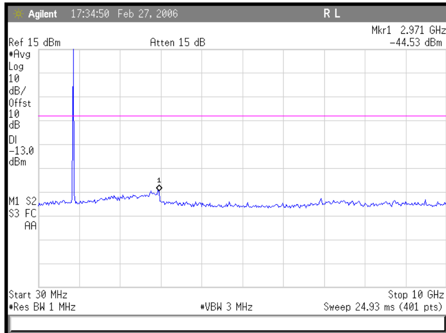
Plot 20. CDMA Downlink Mid CH Conducted Emissions 30 MHz – 10 GHz
