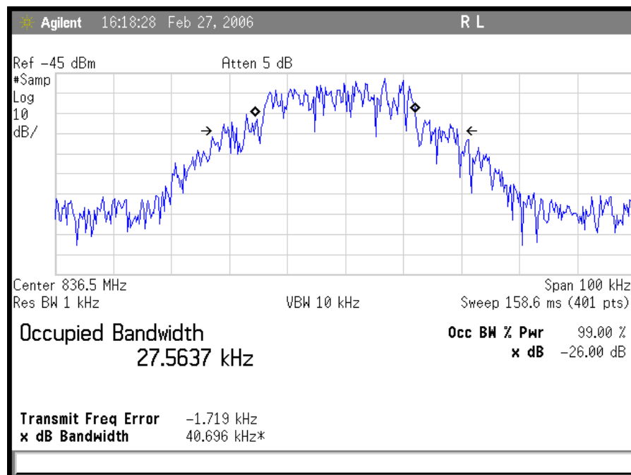
Plot 4. AMPS Uplink Output
