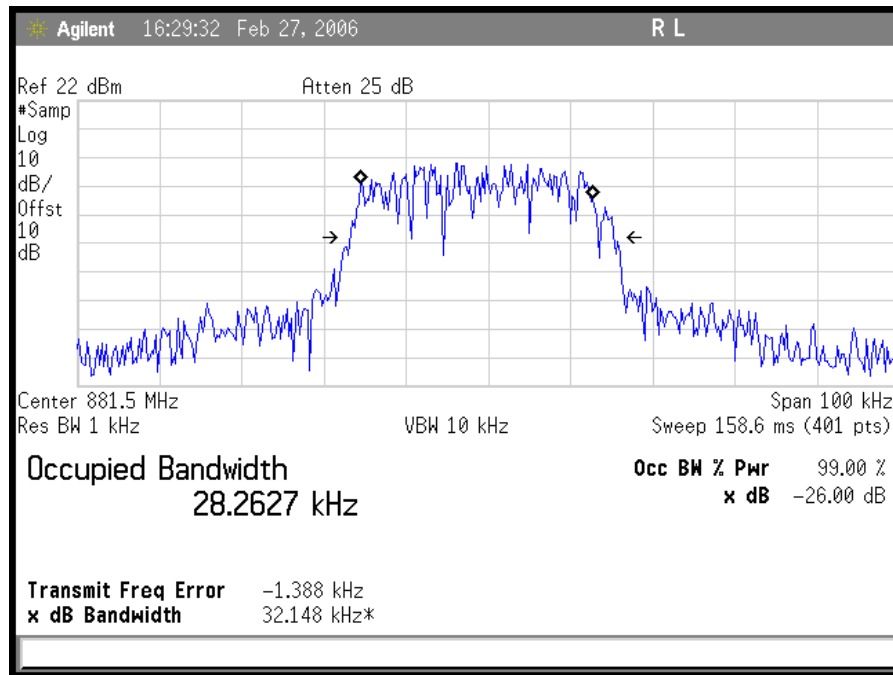
Plot 9. TDMA Downlink Input
