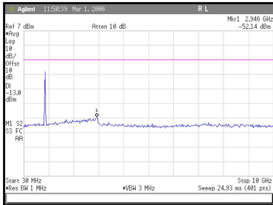
Plot 25. TDMA Downlink Low CH Conducted Emissions 30 MHz – 10 GHz
