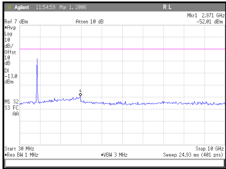
Plot 13. AMPS Downlink Low CH Conducted Emissions 30 MHz – 10 GHz
