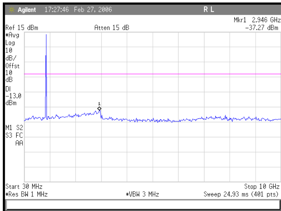
Plot 14. AMPS Downlink Mid CH Conducted Emissions 30 MHz – 10 GHz
