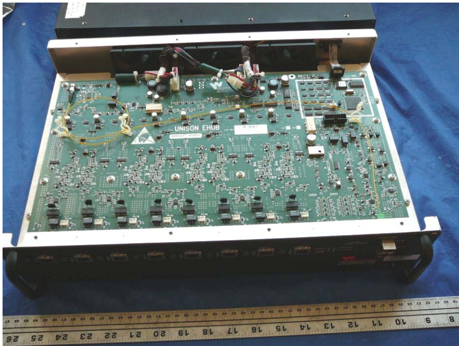
EUT PCB Assembly Top view – EHub
