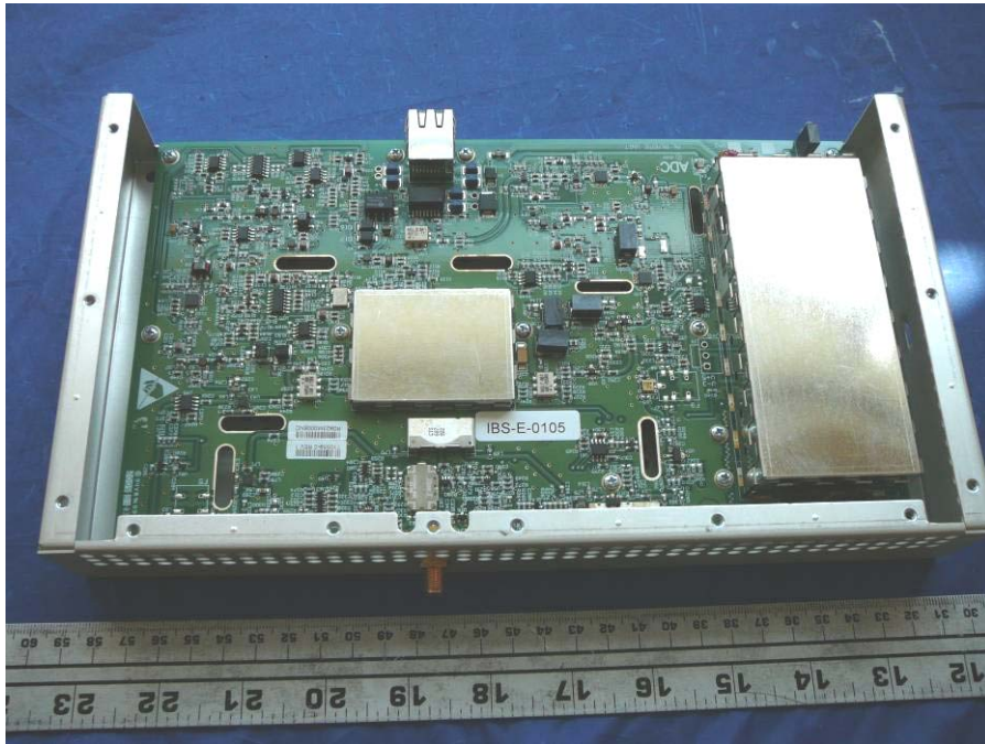
EUT Case off view - RUA
