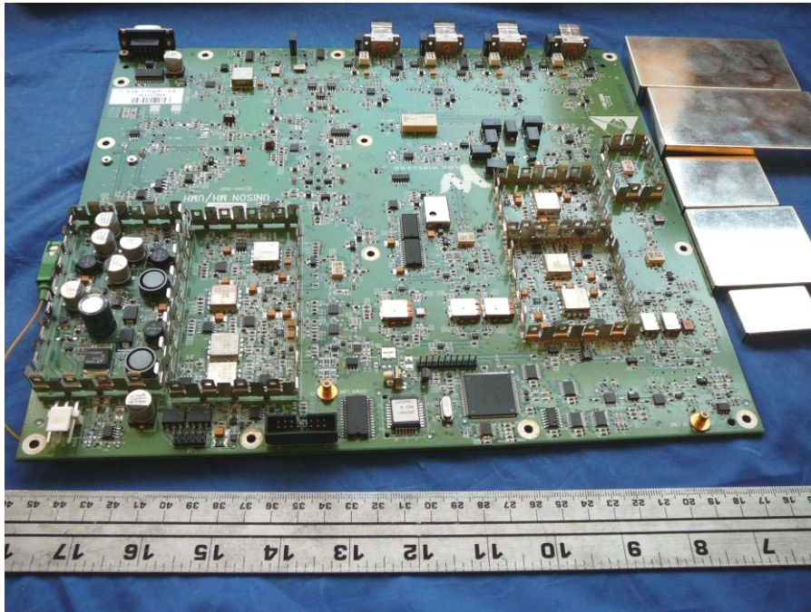
EUT PCB Assembly (Without Shielding) Top View – Main Hub
