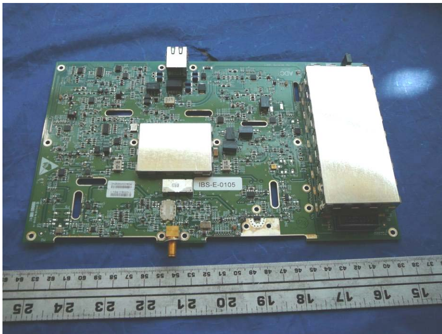
EUT PCB Assembly (With Shielding) Top View - RUA
