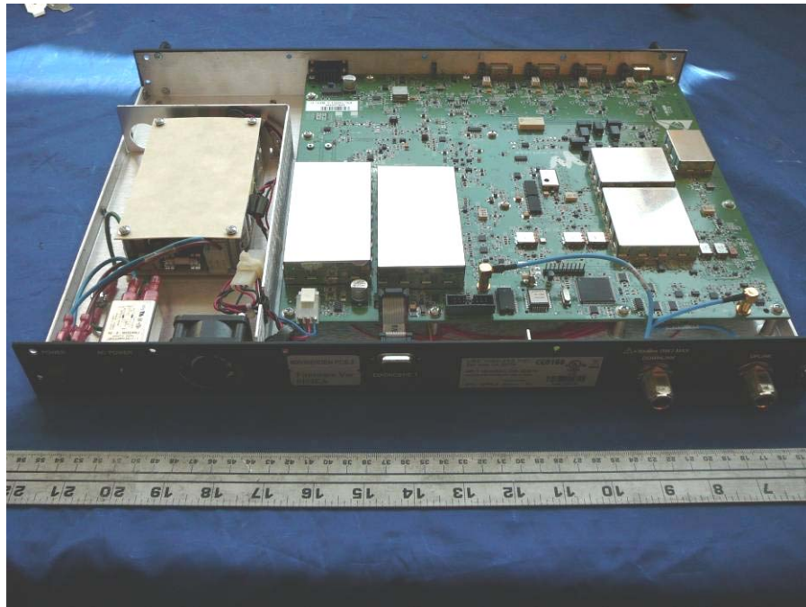
EUT Case Off view – Main Hub
