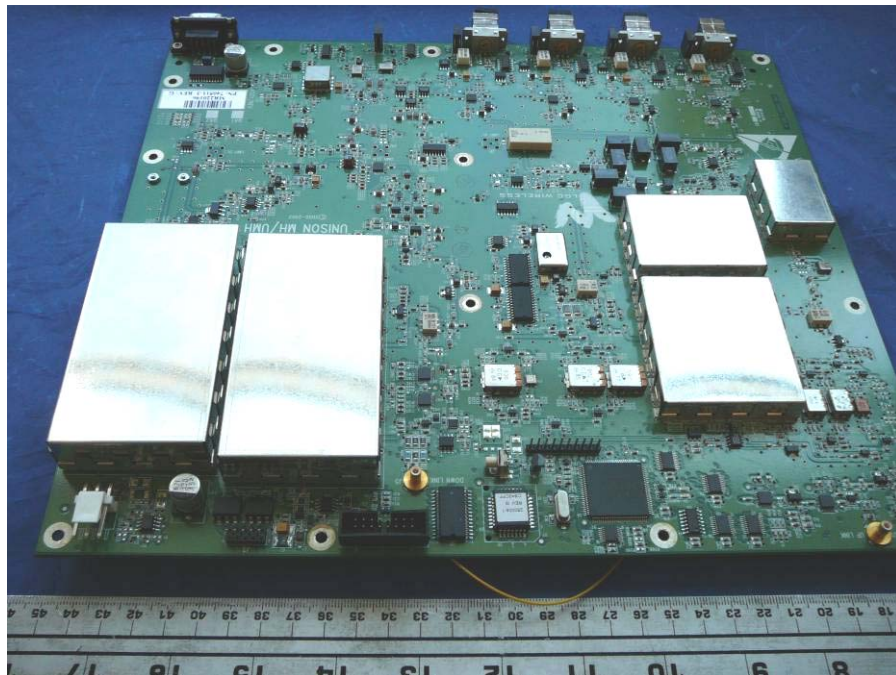
EUT PCB Assembly (With Shielding) Top View – Main Hub
