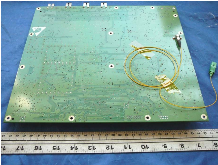
EUT PCB Assembly Bottom View – Main Hub
