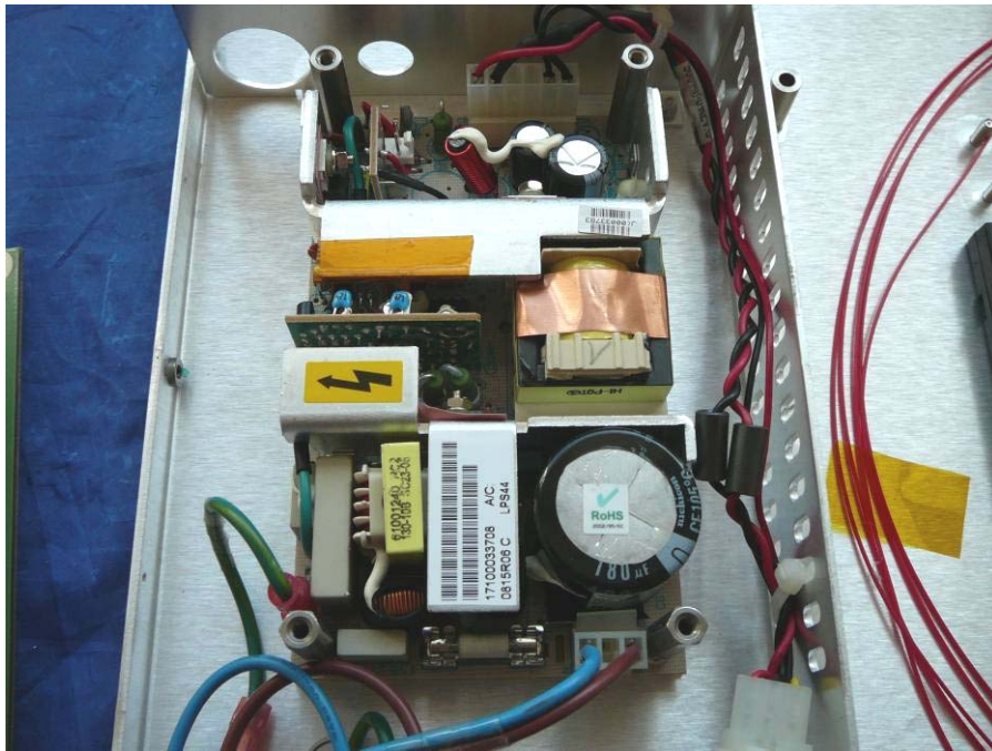
EUT PCB Power Supply Top View – Main Hub
