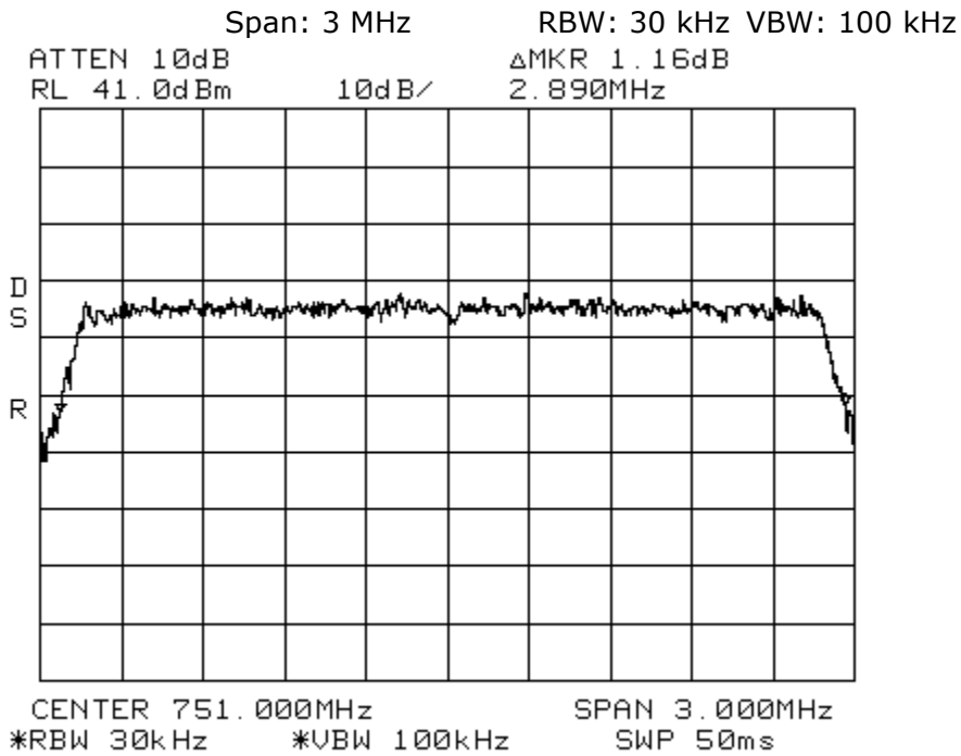
Occupied Bandwidth LTE 3 MHz Channel Bandwidth_Signal_Out Spectrum 700 MHz Upper C Path 2
