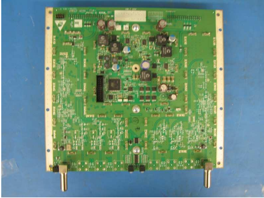
PCB IF Assembly Bottom View without shielding-SRAU
