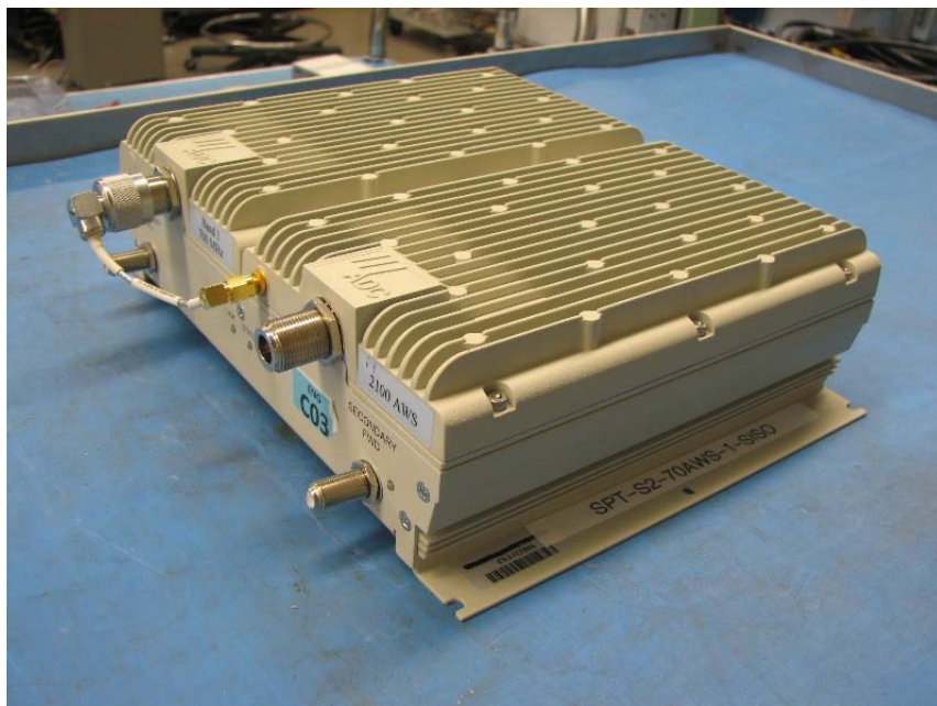
Side View 1
