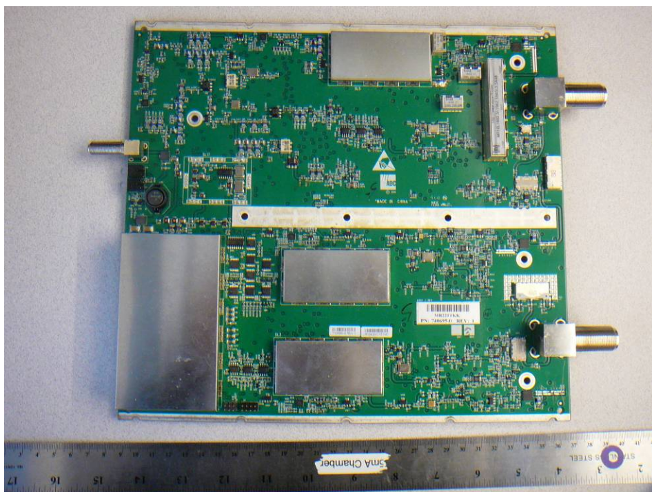
EUT Main PCB (with RF Shield) Top View – RAU
