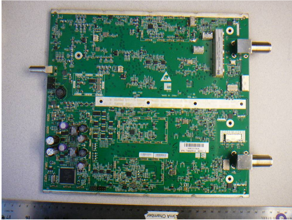
EUT Main PCB (with RF Shield) Bottom View – RAU
