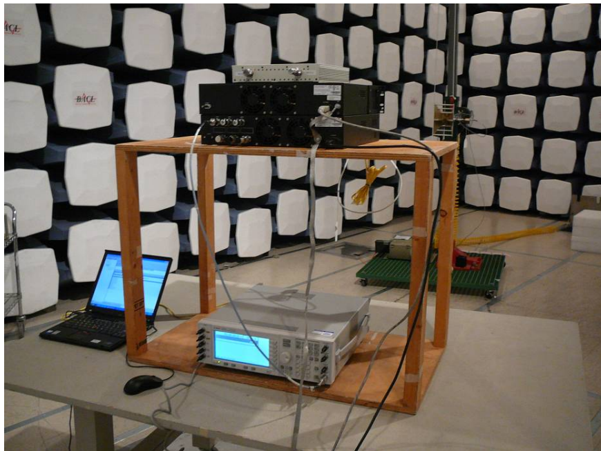
Radiated Emissions above 1GHz- Rare View
