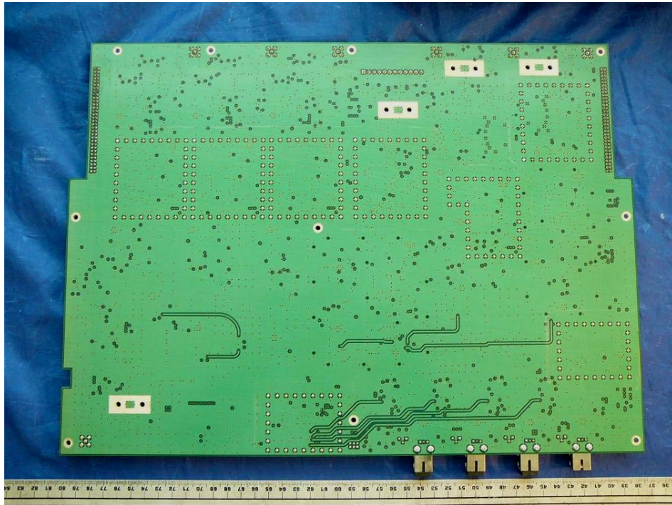
EUT PCB-2 Assembly Top View – Main HUB
