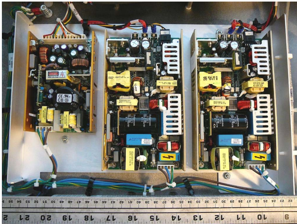
EUT PCB Power Supplies Top View – EHUB
