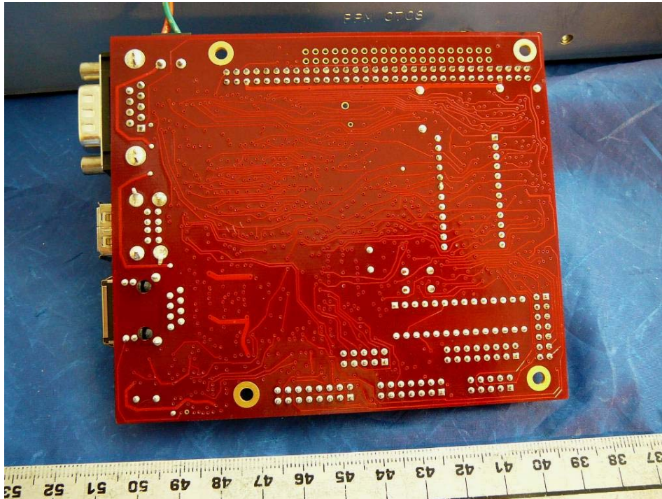
EUT PCB-3 Assembly Bottom View – Main HUB
