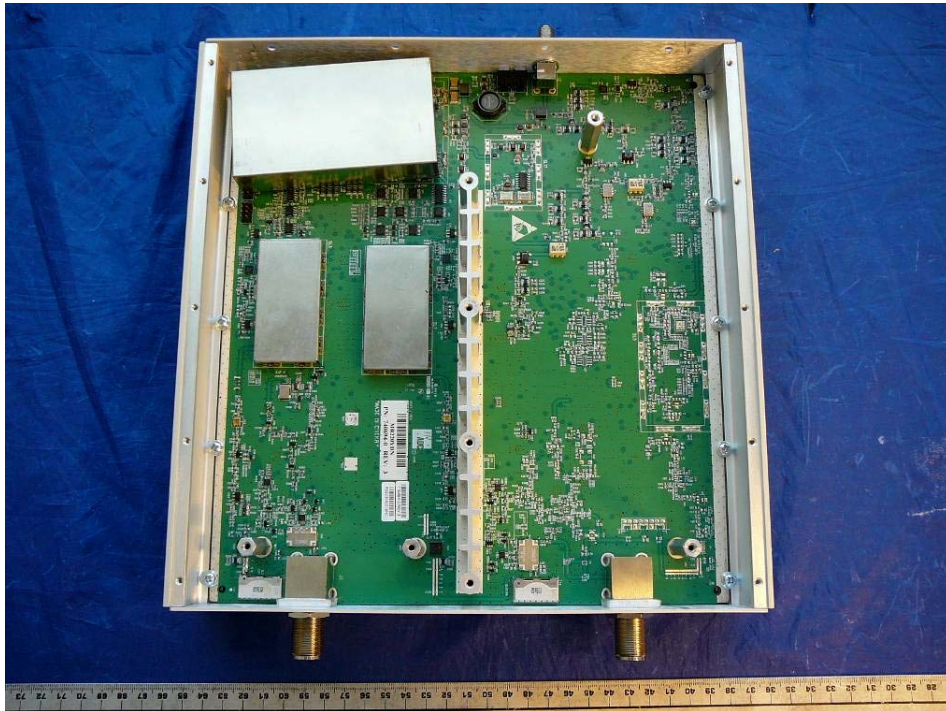
EUT Case off view - RUA
