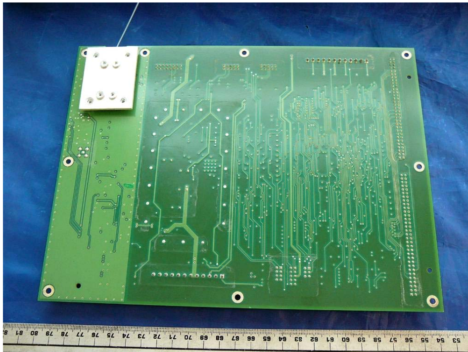
EUT PCB-3 Assembly Top View – Main HUB
