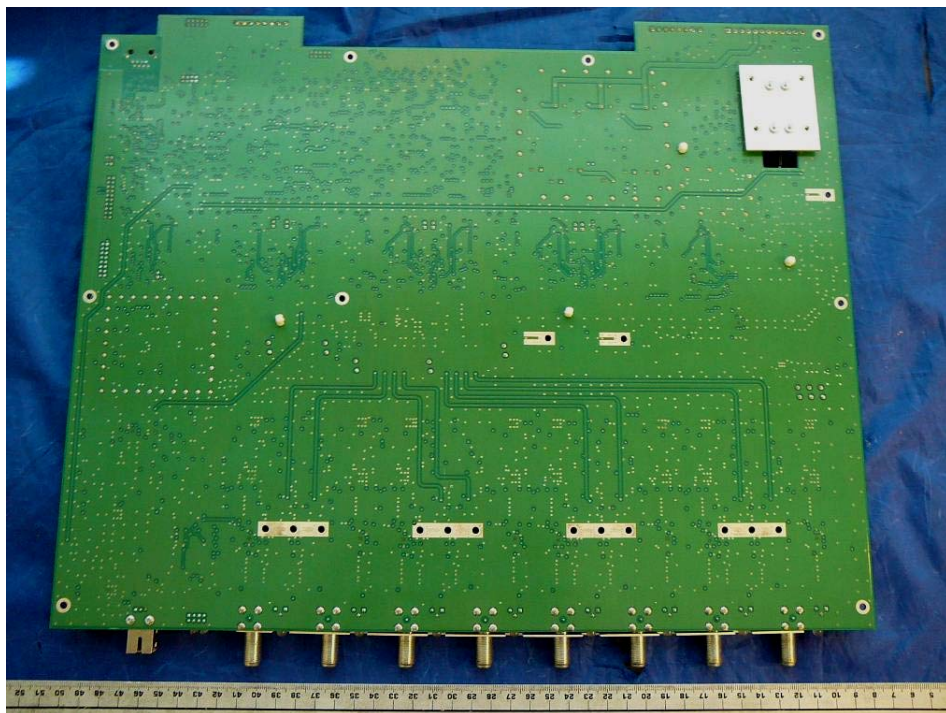
EUT PCB Assembly Bottom View – EHUB
