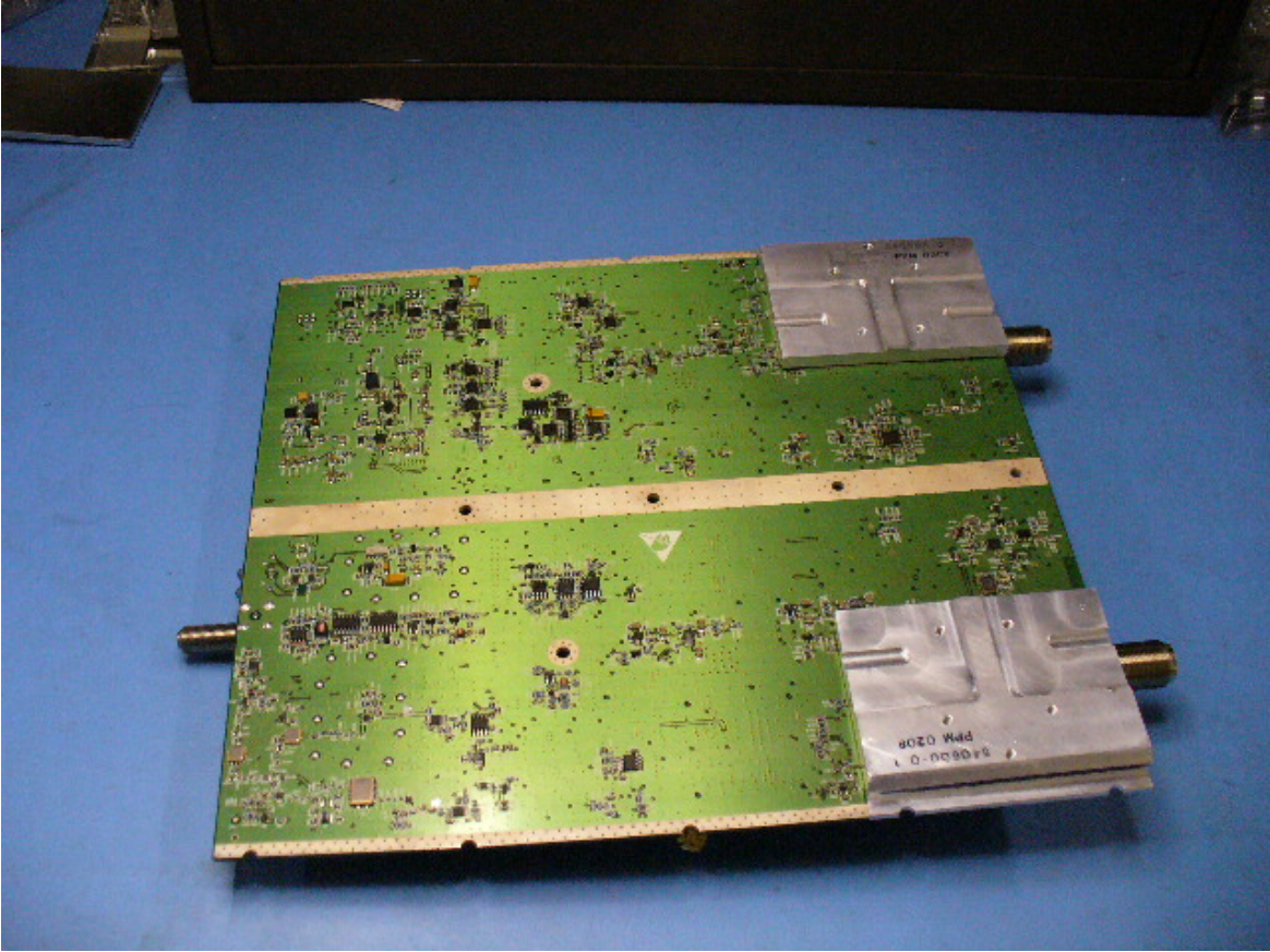
InterReach® Fusion Remote Access Unit Bottom View - 1
