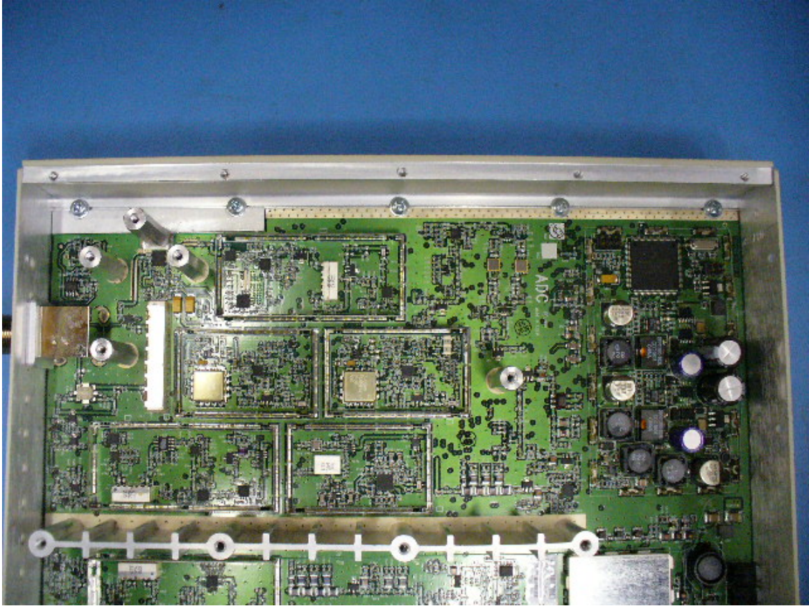
InterReach® Fusion Remote Access Unit Top View - 3
