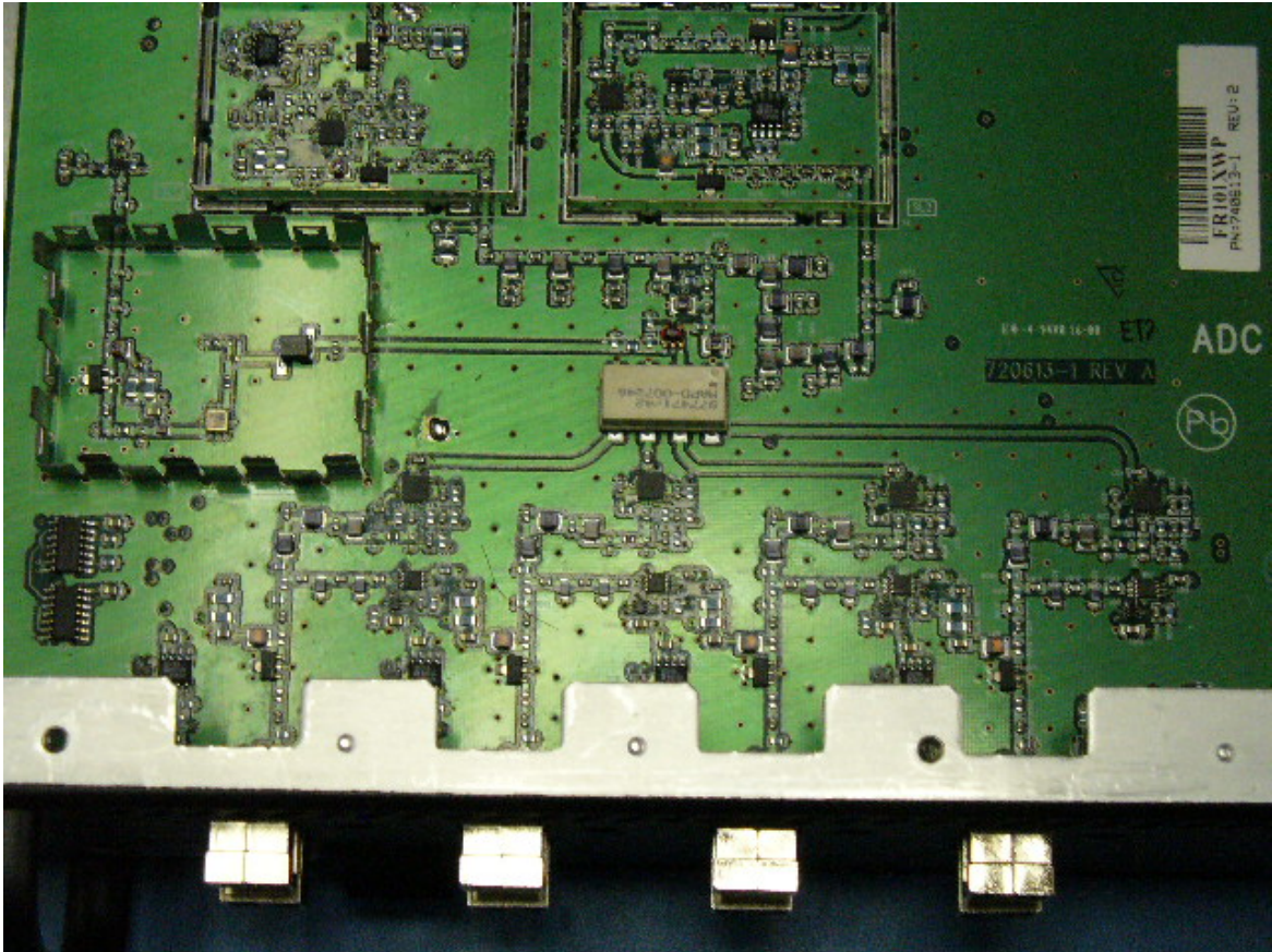
InterReach® Fusion Main Hub Top View - 1
