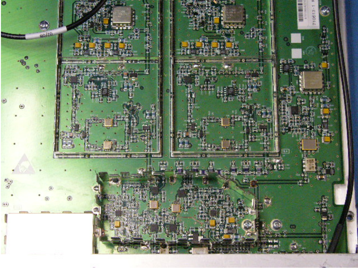
InterReach® Fusion Main Hub Top View - 2
