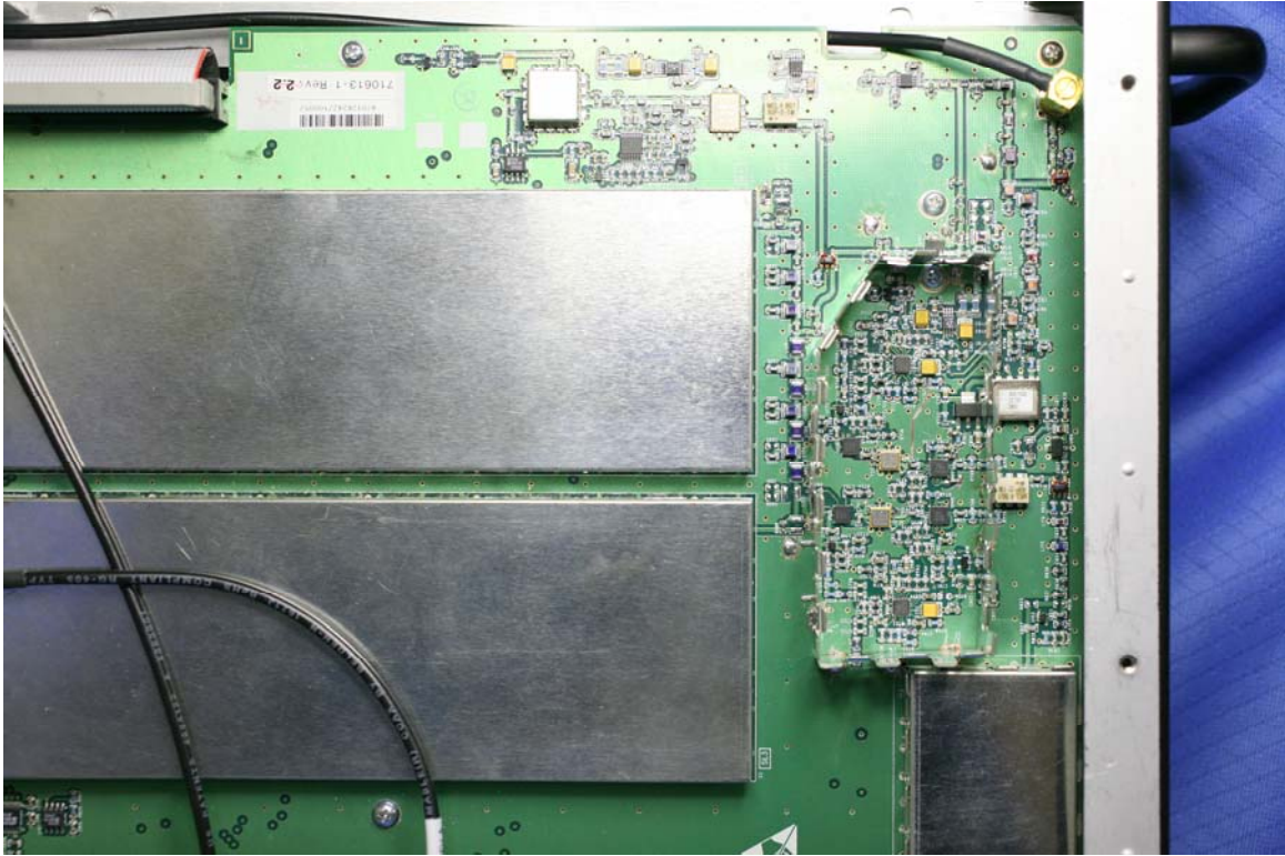
InterReach® Fusion Main Hub Top View – 4
