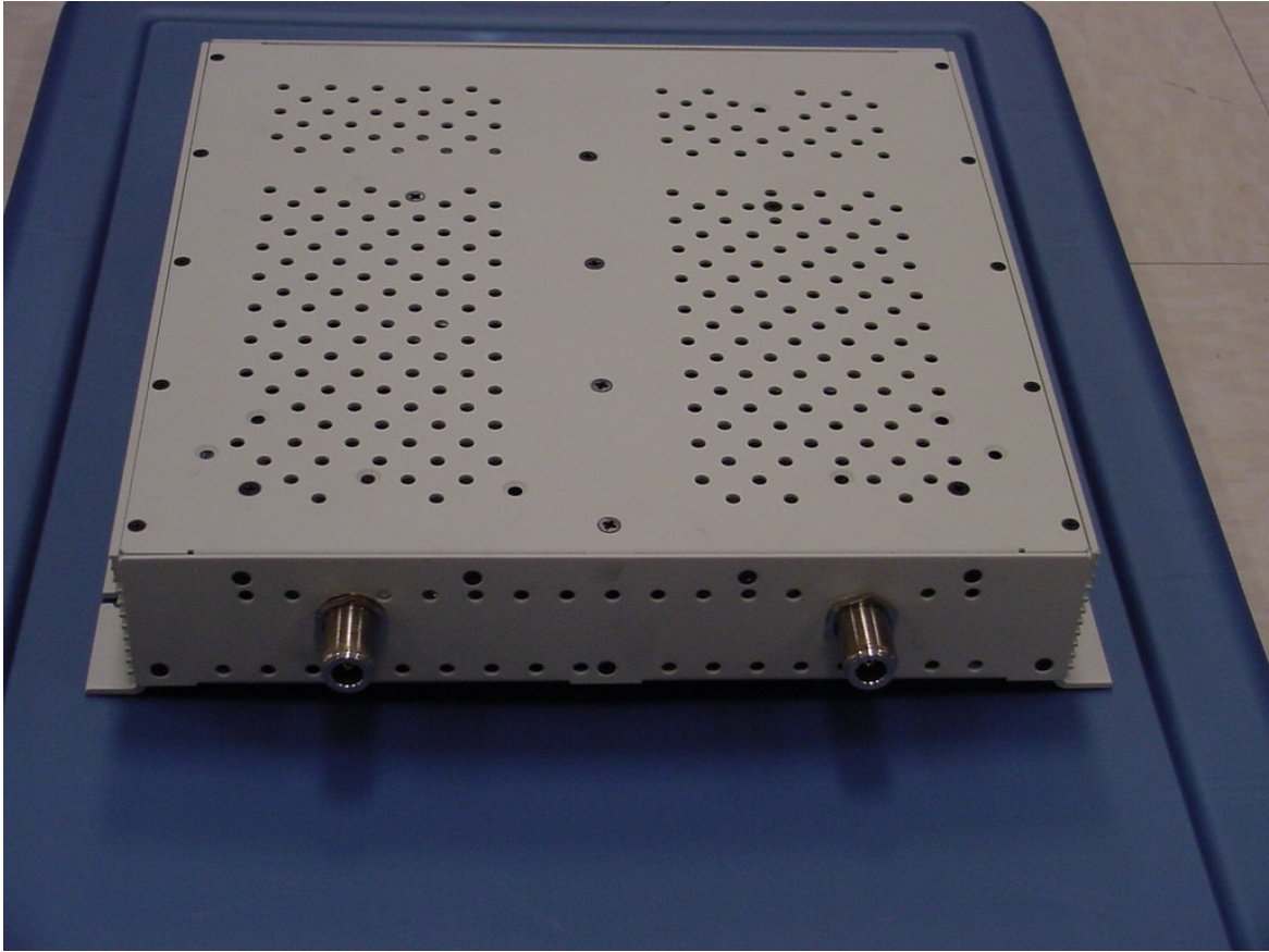
InterReach® Fusion Remote Access Unit Rear View
