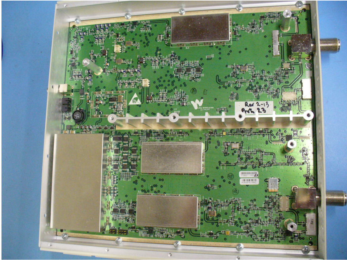
InterReach® Fusion Remote Access Unit Open Top View
