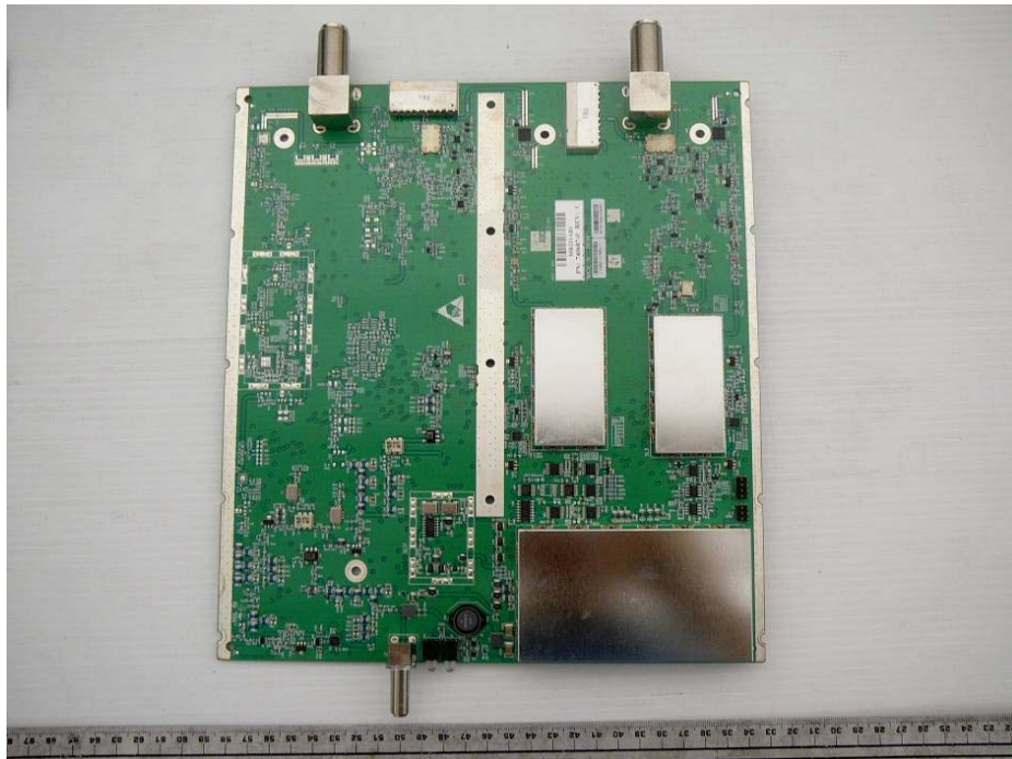
EUT – RAU Main Board Top View
