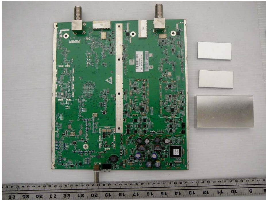
EUT – RAU Main Board Bottom View
