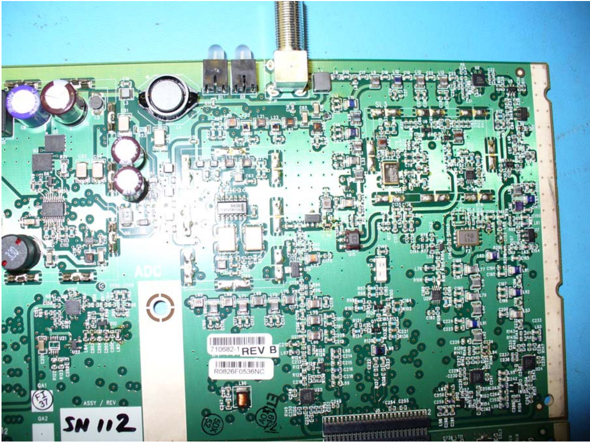
InterReach® Fusion Remote Access Unit Top View 1 – Universal Section
