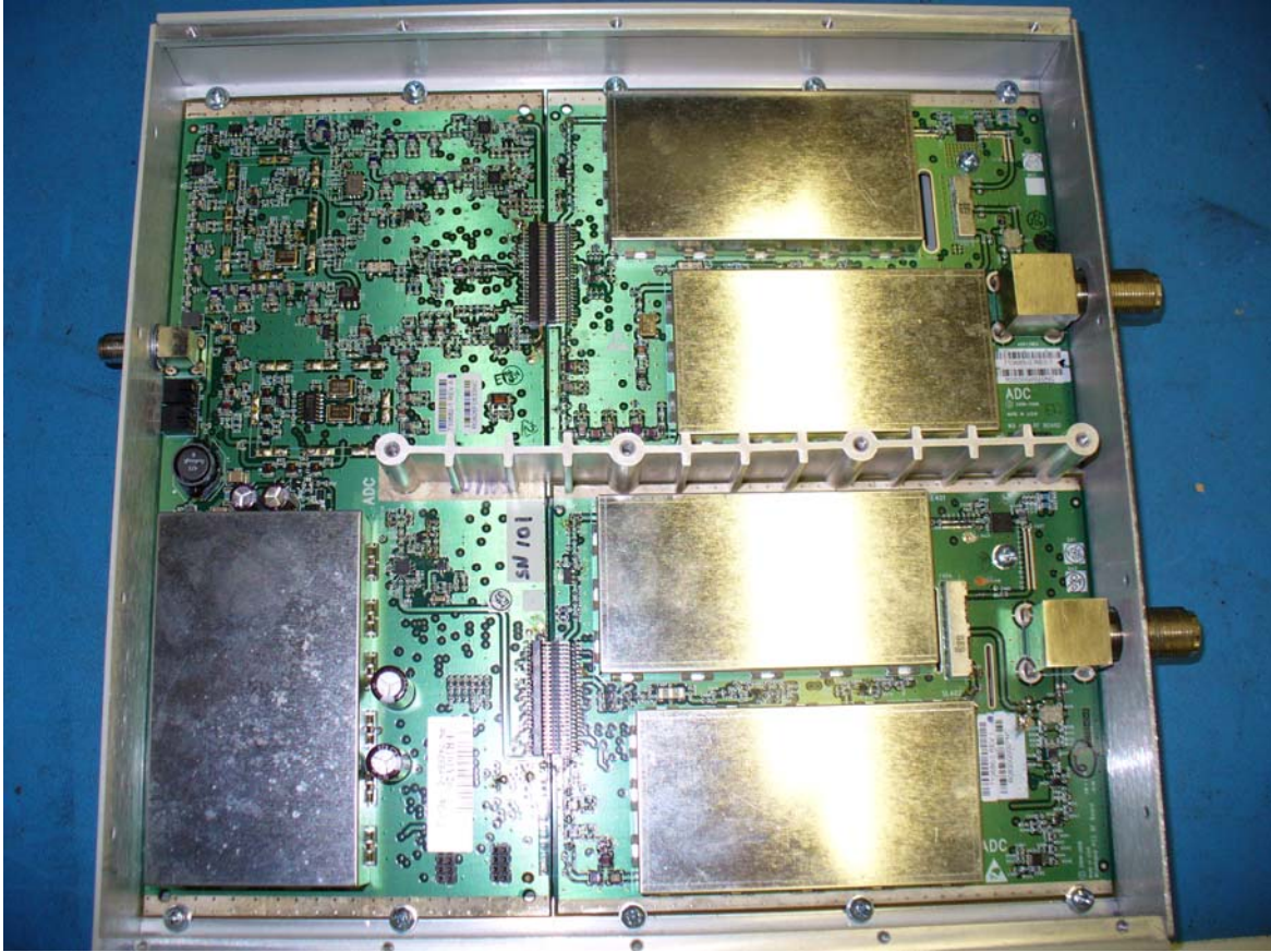
InterReach® Fusion Remote Access Unit Top View – Cover Removed
