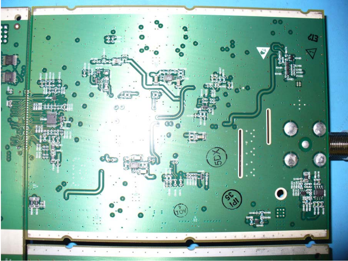
InterReach® Fusion Remote Access Unit Bottom View – PCS Section
