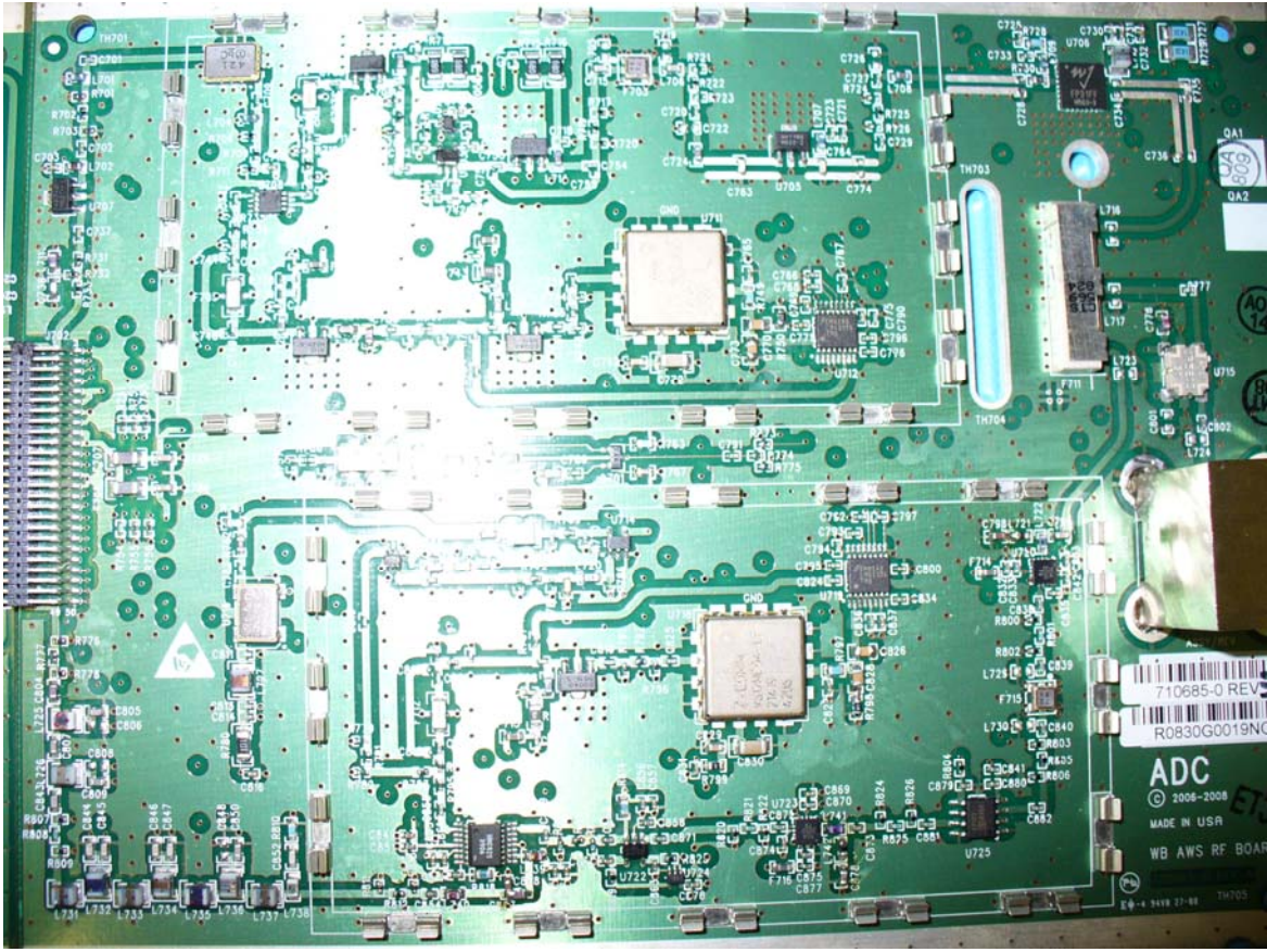
InterReach® Fusion Remote Access Unit Top View – AWS Section
