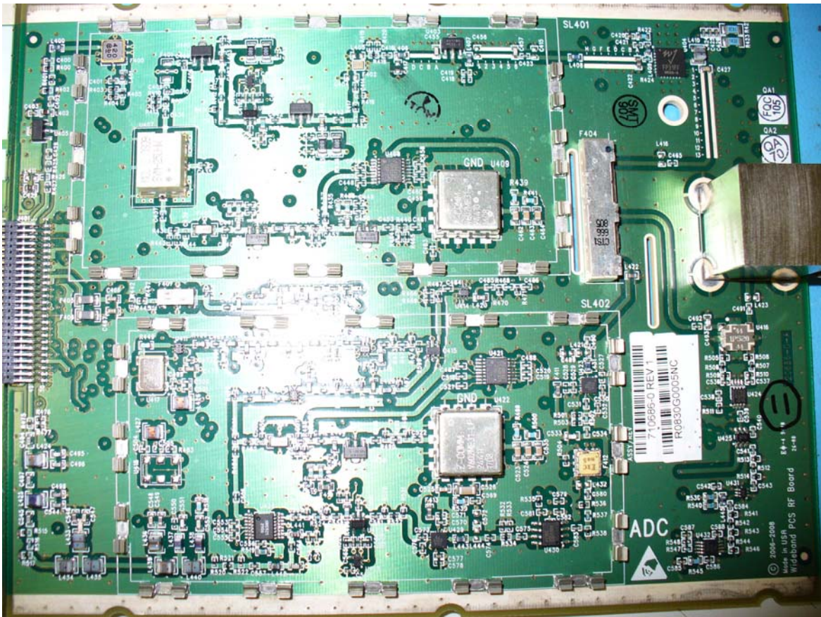
InterReach® Fusion Remote Access Unit Top View – PCS Section
