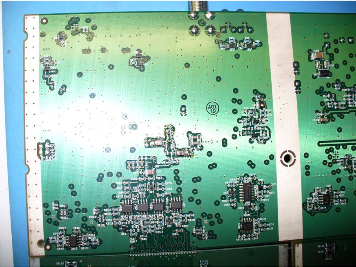
InterReach® Fusion Remote Access Unit Bottom View 2 – Universal Section
