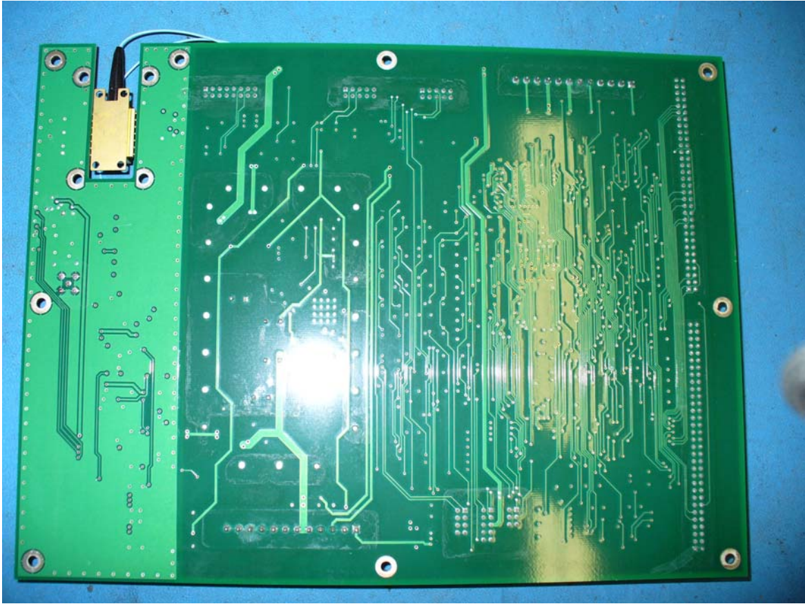
InterReach® Fusion Main Hub Bottom View – Digital Board
