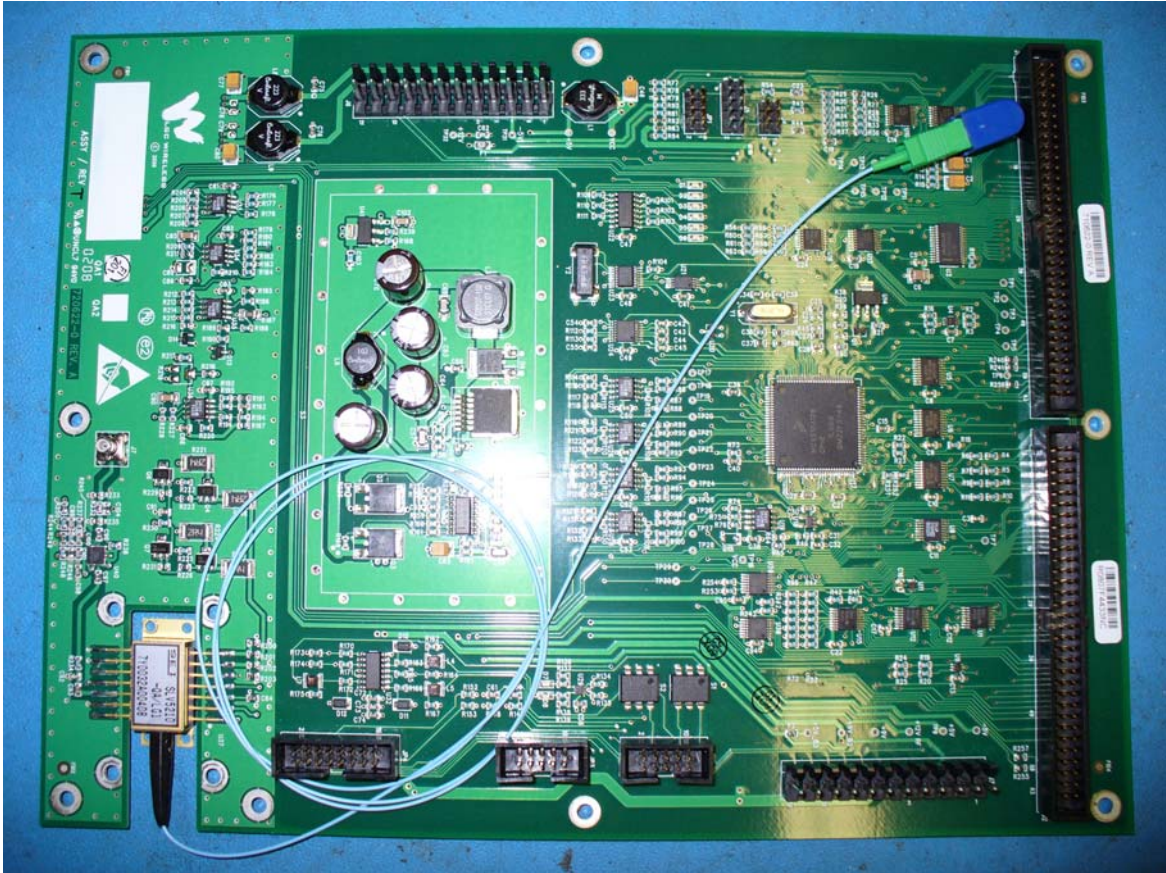
InterReach® Fusion Main Hub Top View – Digital Board
