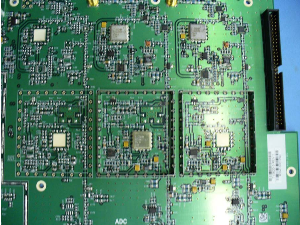
InterReach® Fusion Main Hub Top View 1 – Downlink RF
