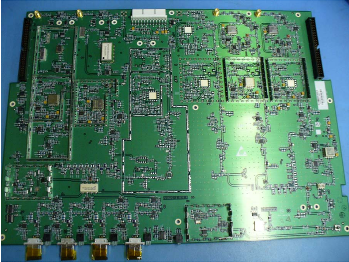
InterReach® Fusion Main Hub Top View – RF Board
