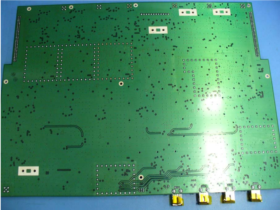
InterReach® Fusion Main Hub Bottom View – RF Board
