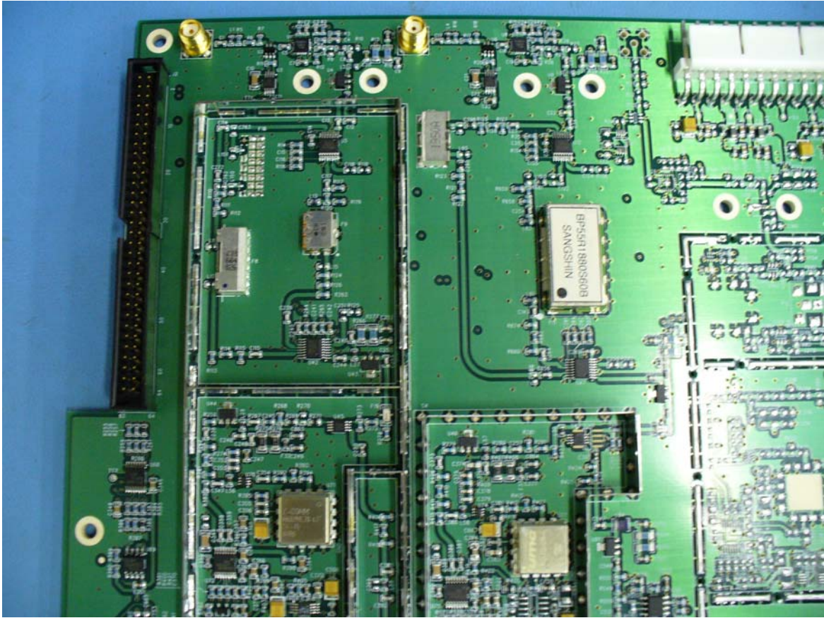
InterReach® Fusion Main Hub Top View 1 – Uplink RF
