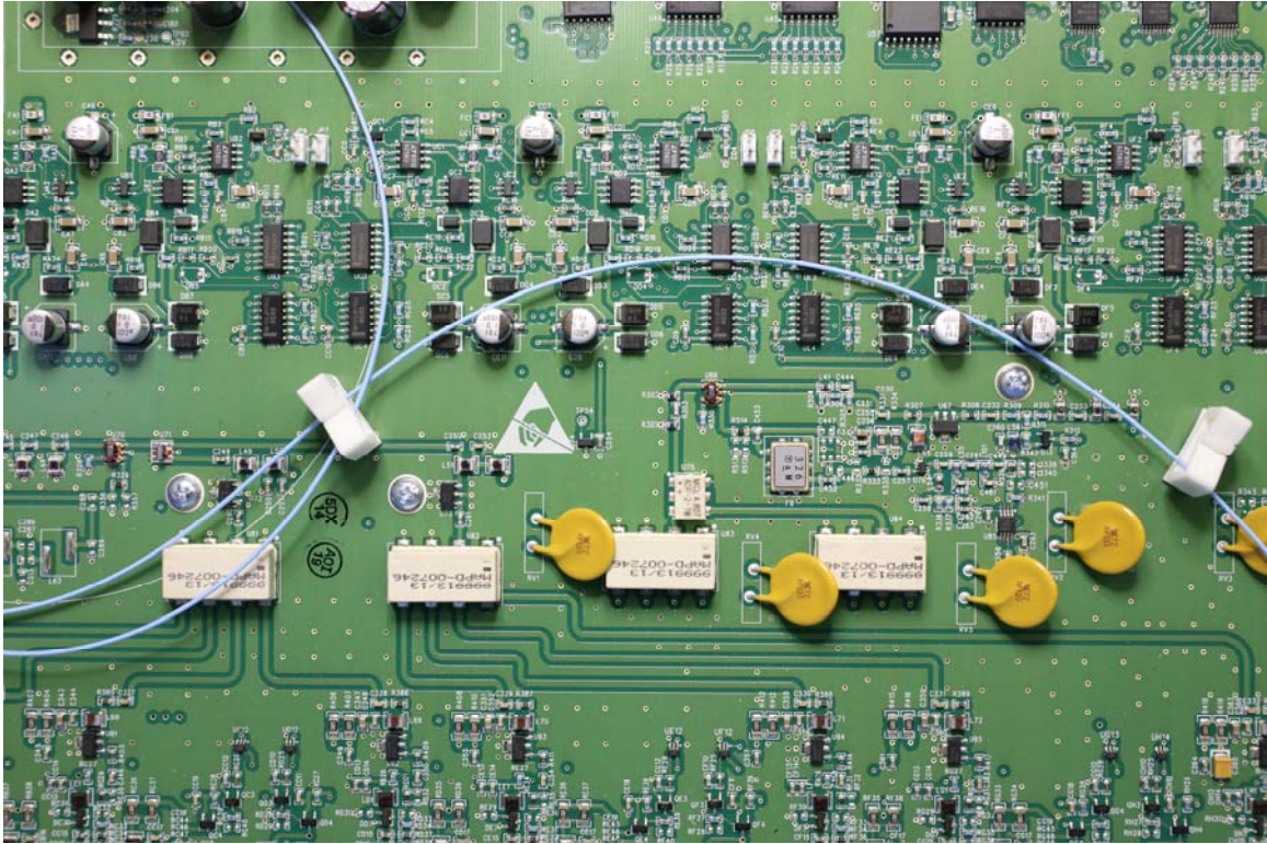
InterReach® Fusion Expansion Hub Top View - 9
