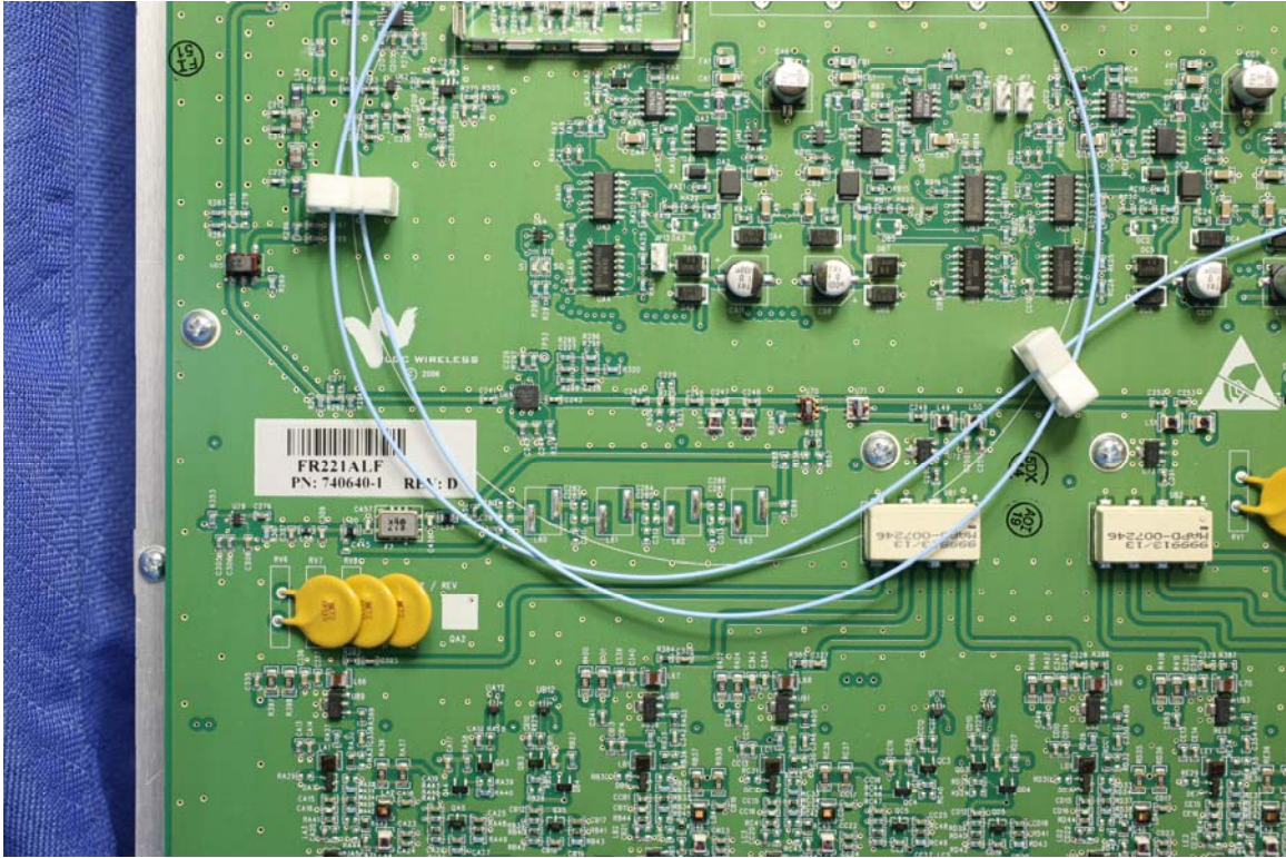
InterReach® Fusion Expansion Hub Top View - 2
