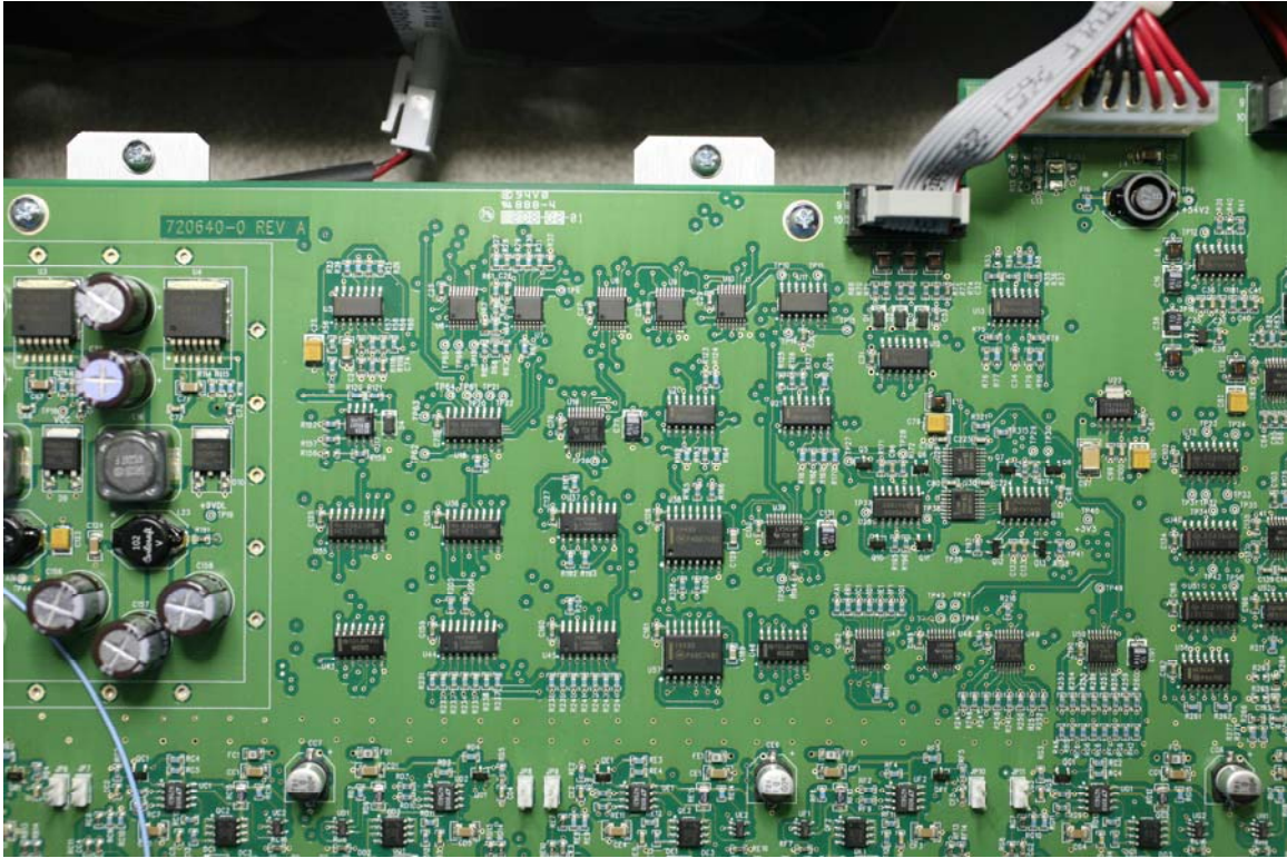
InterReach® Fusion Expansion Hub Top View - 8
