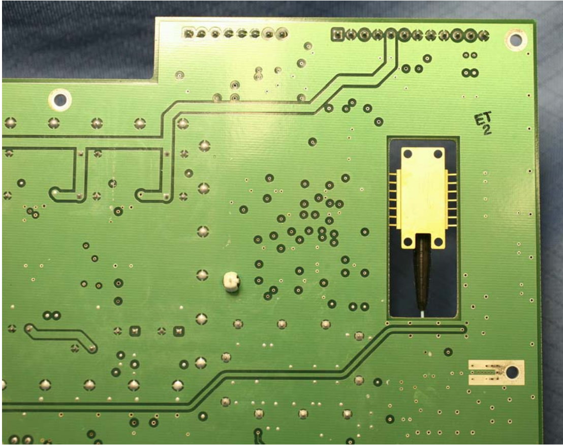
InterReach® Fusion Expansion Hub Bottom View - 2
