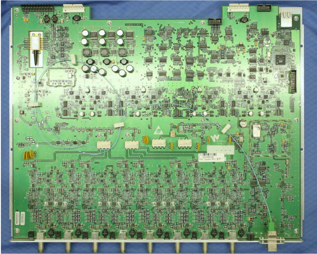
InterReach® Fusion Expansion Hub Top View
