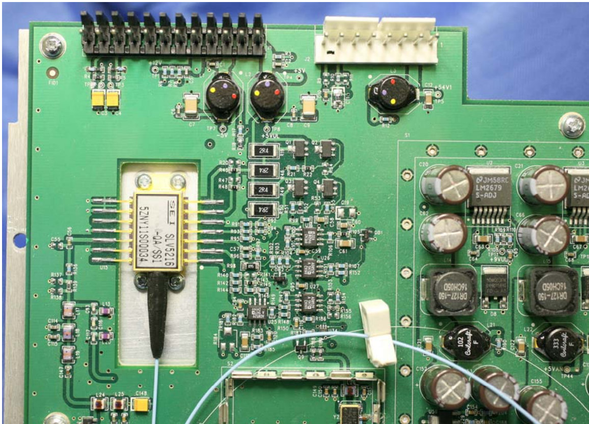
InterReach® Fusion Expansion Hub Top View - 1
