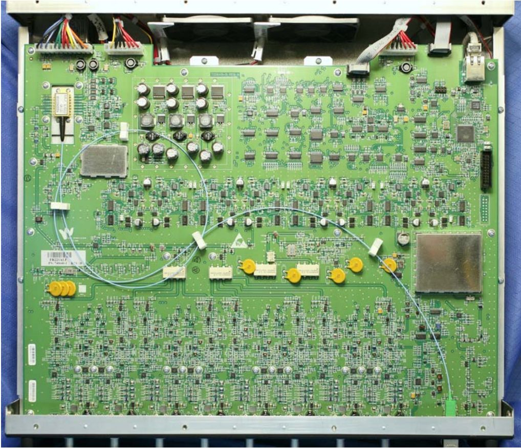
InterReach® Fusion Expansion Hub Open Top View
