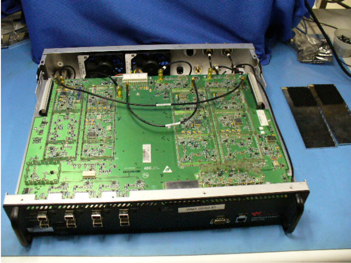
InterReach® Fusion Main Hub Open Top View - 1
