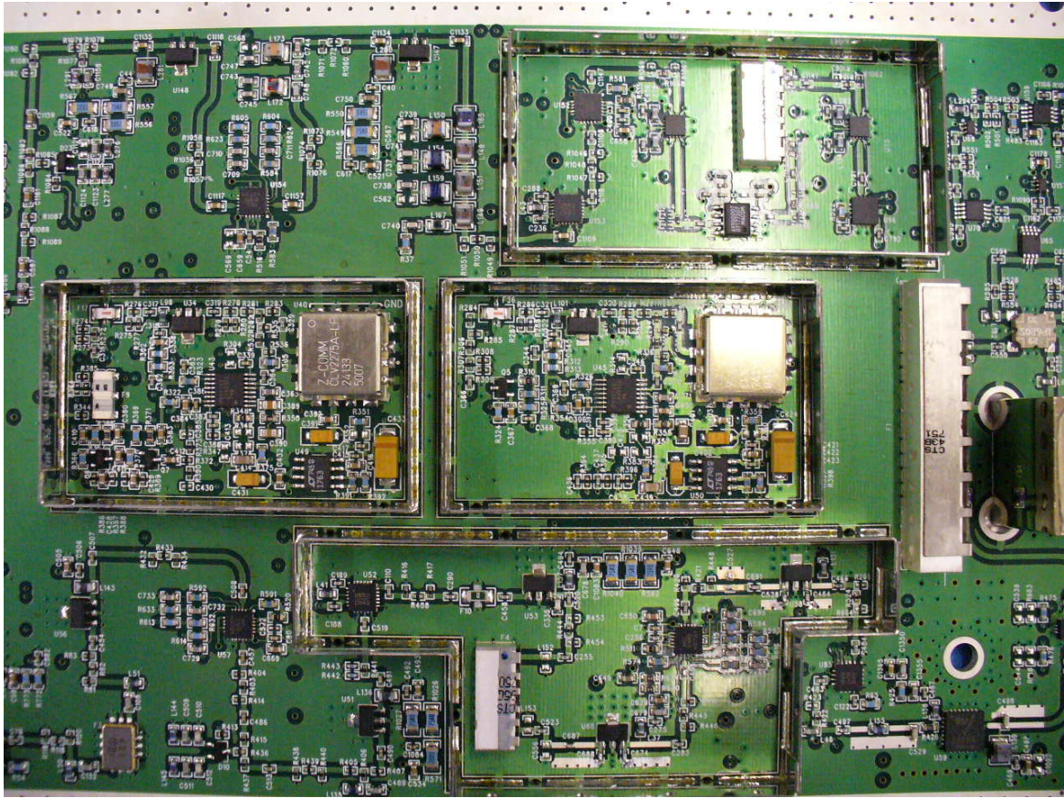
InterReach® Fusion Remote Access Unit Top View - 5
