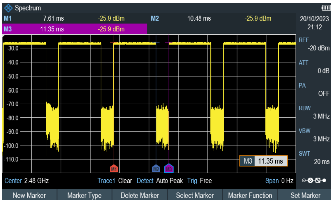
Time-domain plot for Bluetooth transmission signal
