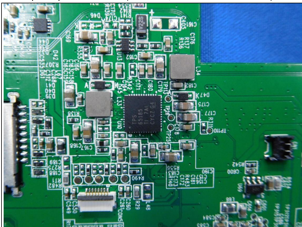
panel power IC No. 1 (Brand: TI, Model: TPS65185RSL)
