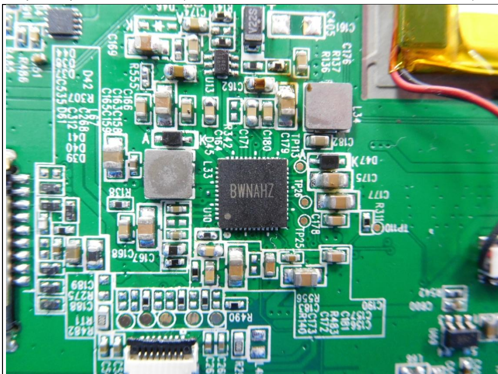
panel power IC No. 2 (Brand: SILERGY, Model: SY7636ARMC)
