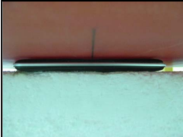
The Bottom of the EUT face to the phantom with 0mm-separation distance.
