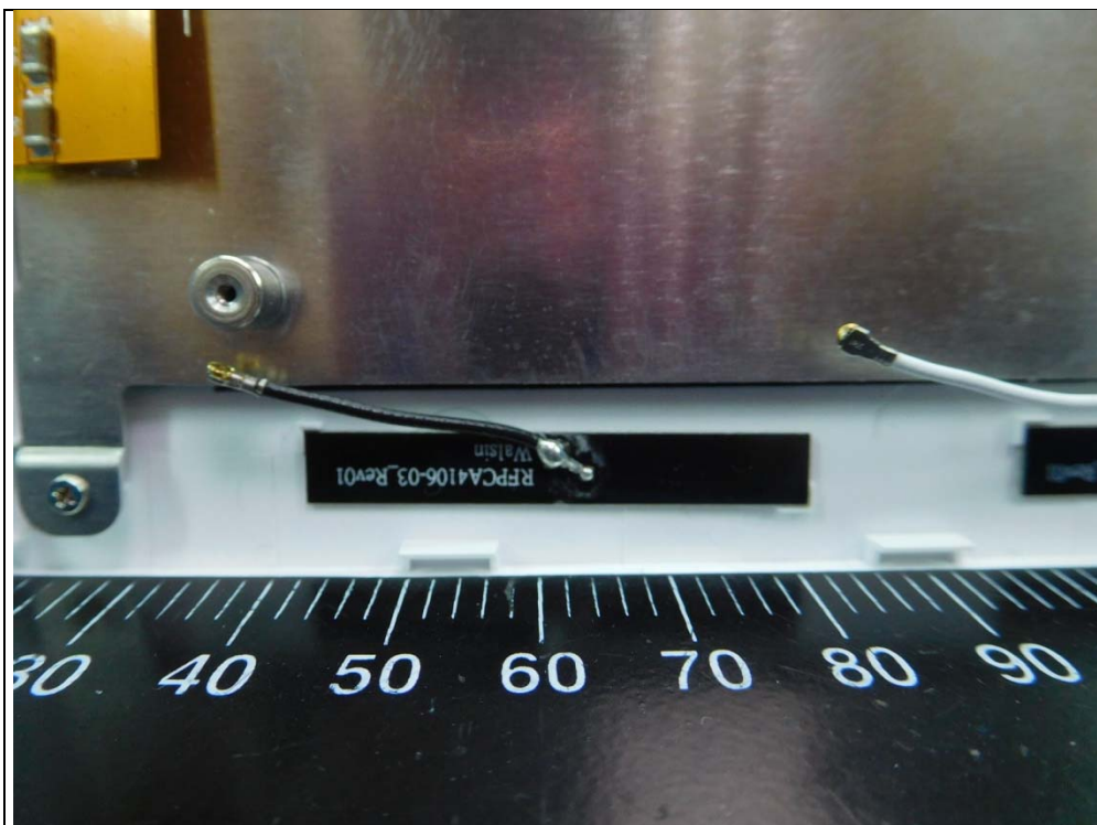
Zigbee Antenna
