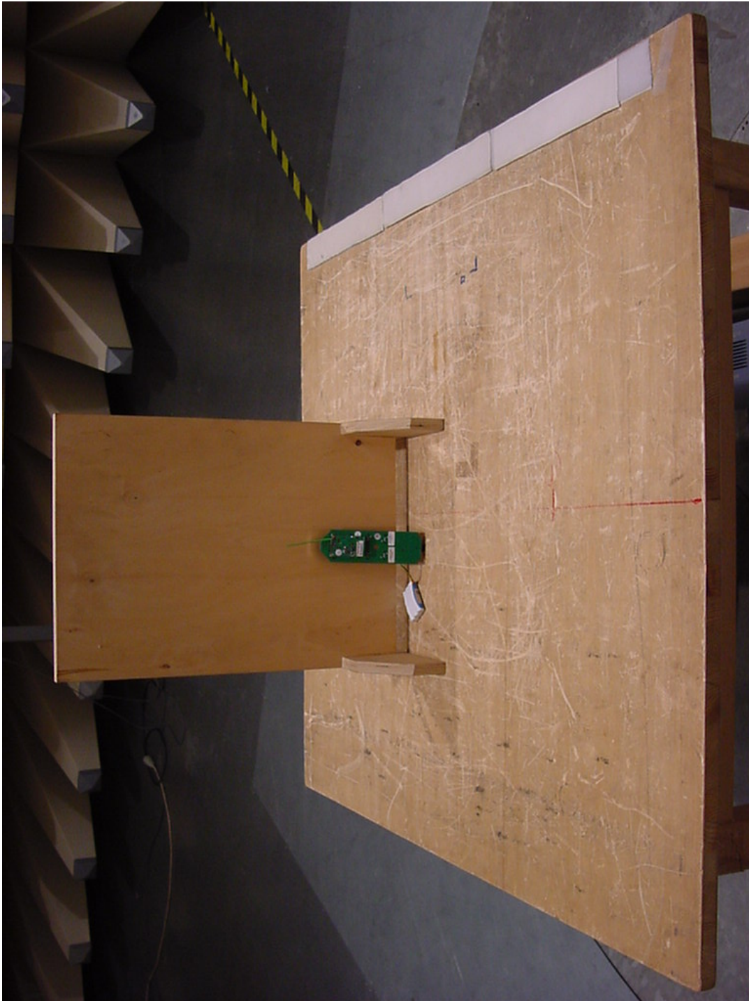
Photo 2 (Radiated Emissions):
