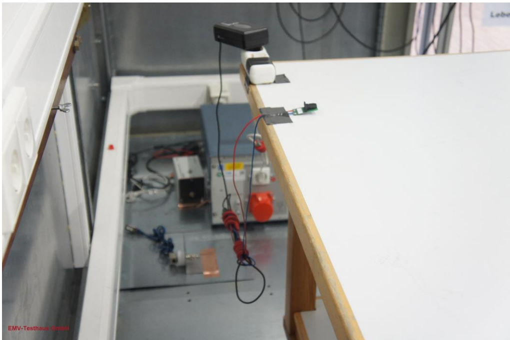
Picture 2: EUT test setup conducted emission test (rear view)
