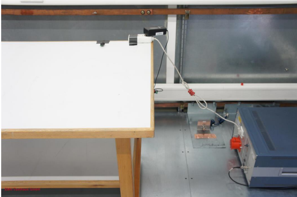
Picture 1: EUT test setup conducted emission test (front view)
