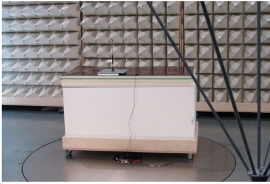
Radiated Setup A, Monopole MU 911-LX
