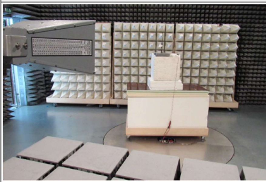
Radiated Setup C, Monopole MU 911-LX
