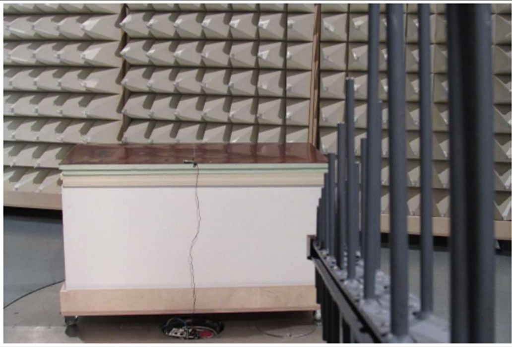
Radiated Setup 200 MHz to 1 GHz
