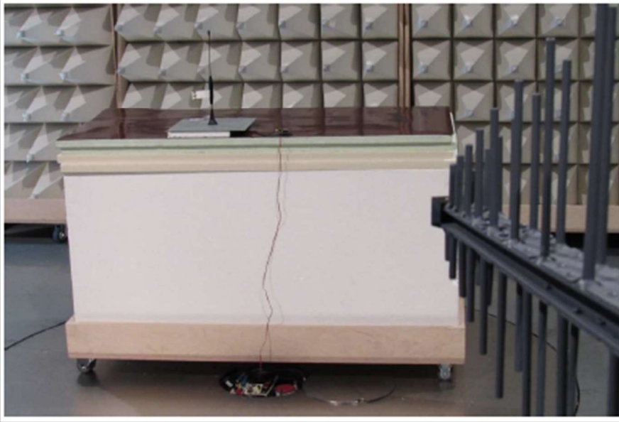
Radiated Setup B, Monopole MU 911-LX
