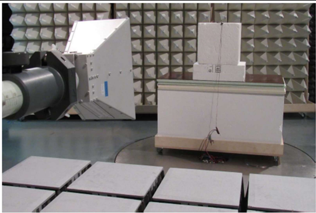
Radiated Setup upper 1 GHz
