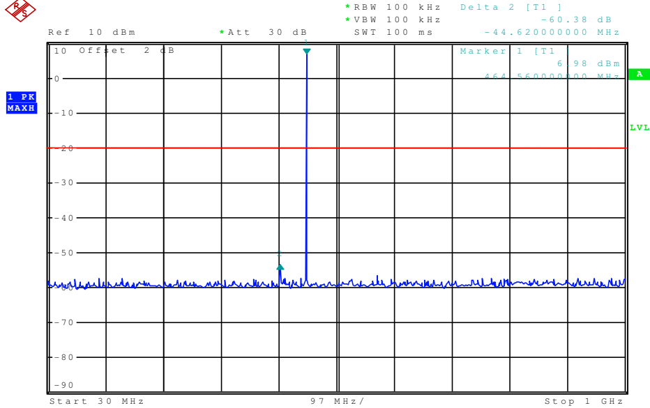
Plot 1: 30 MHz – 1 GHz (465.01875 MHz)
