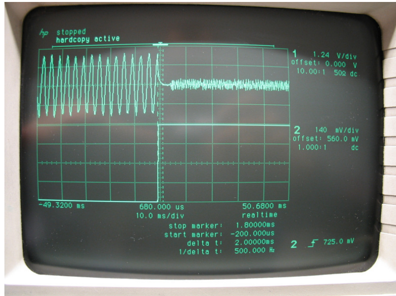
Plot 6: 469.98125 MHz (Switch off)
