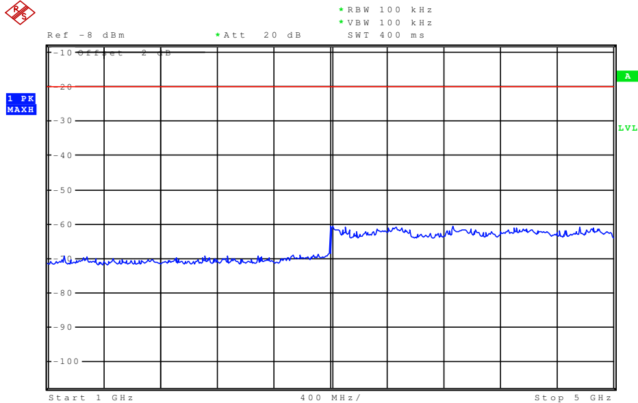
Plot 2: 1 GHz – 5 GHz (465.01875 MHz)
