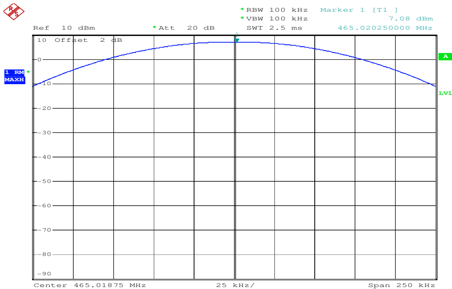
Plot 1: Peak output power 465.01875 MHz (conducted)
