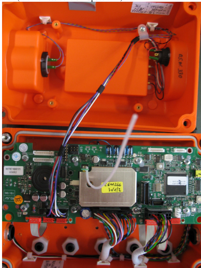
Photo 8: Measuring combination (with remote control "Spectrum")
