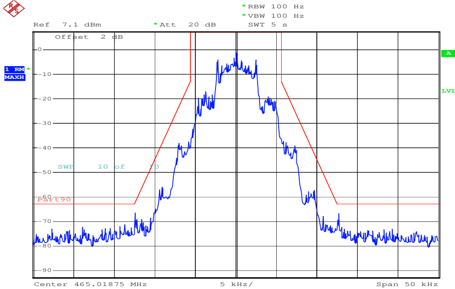
Plot 1: 465.01875 MHz (max. power), modulated with test modulation 12.5 kHz BW
