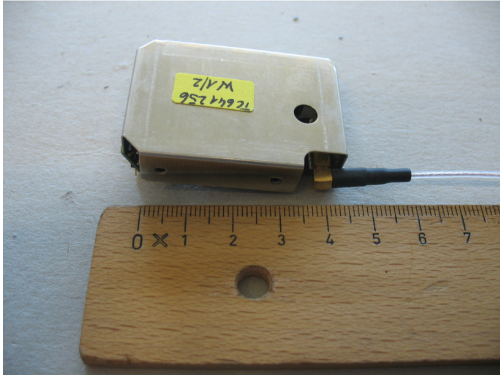
Photo 5: Antenna-connection
