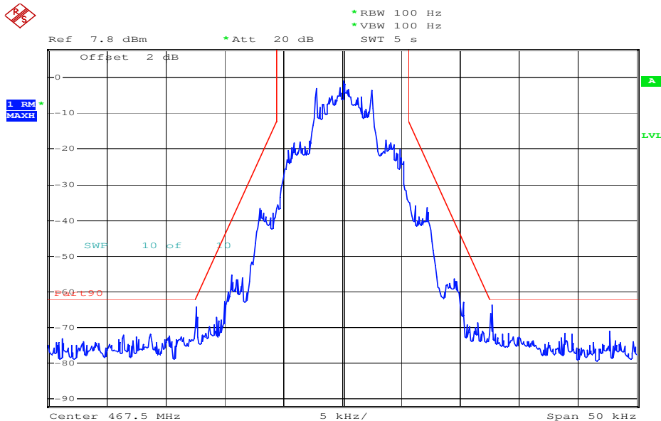
Plot 2: 467.50000 MHz (max. power), modulated with test modulation 12.5 kHz BW
