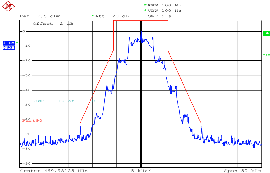
Plot 3: 469.98125 MHz (max. power), modulated with test modulation 12.5 kHz BW
