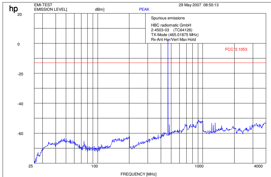
Plot 1: TX-Mode 465.01875 MHz (30 MHz – 4 GHz)
