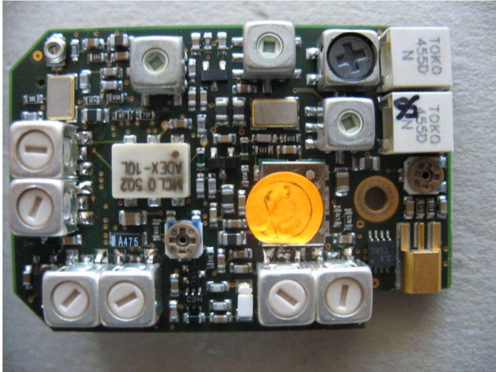
Photo 6: Antenna-connection
