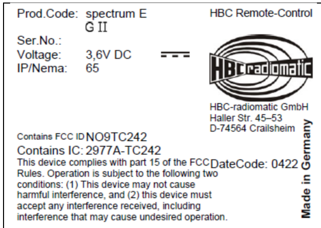
Figure 1: Example type plate of a host device
