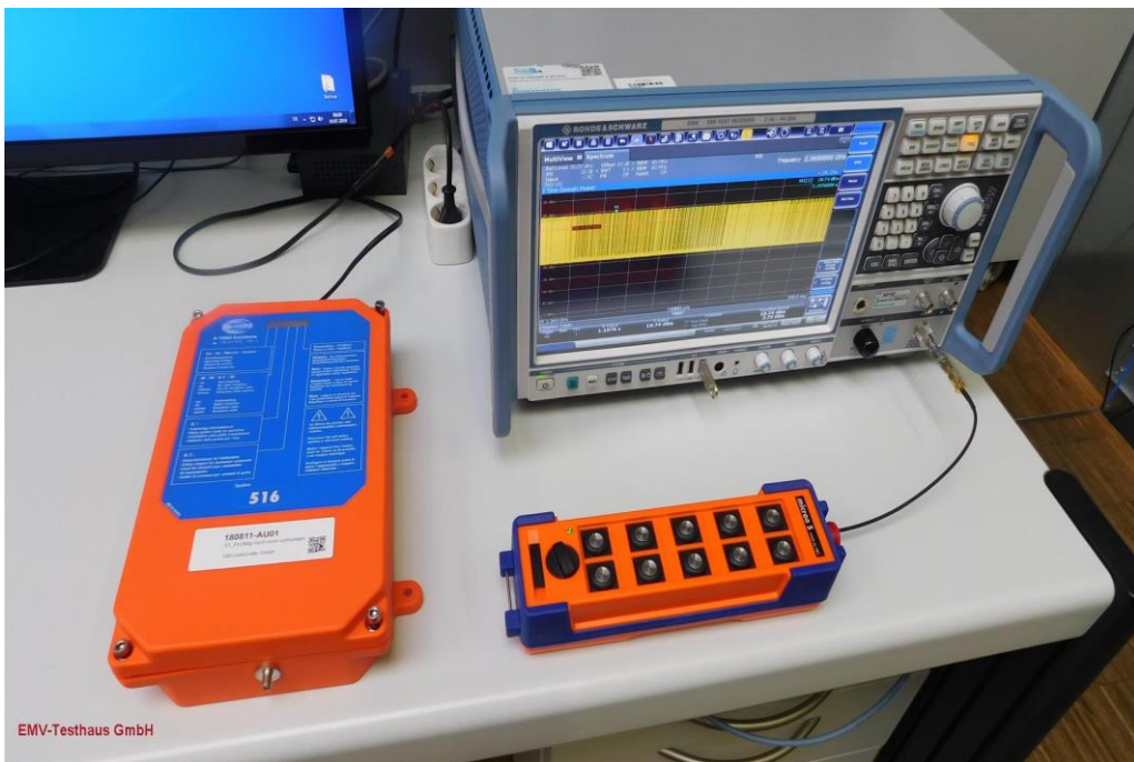
Picture 12: Conducted measurement for RF exposure
