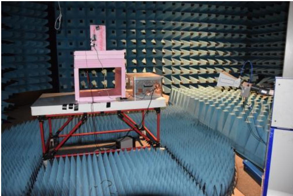
Picture 7: AC, radiated emission test 1 GHz – 17 GHz – position Y (front view)
