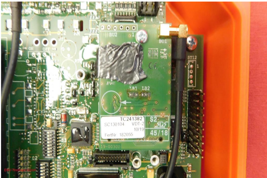
Picture 16: Detailed view of module in companion device
