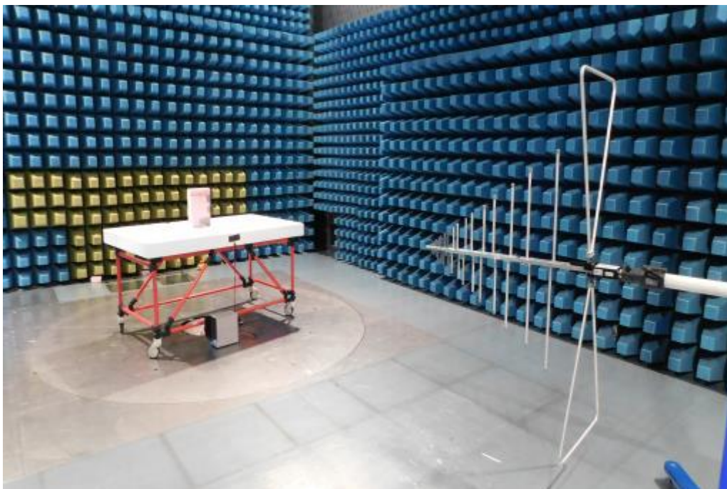
Picture 6: SAC, radiated emission test 30 MHz – 1 GHz – position Y (back view)
