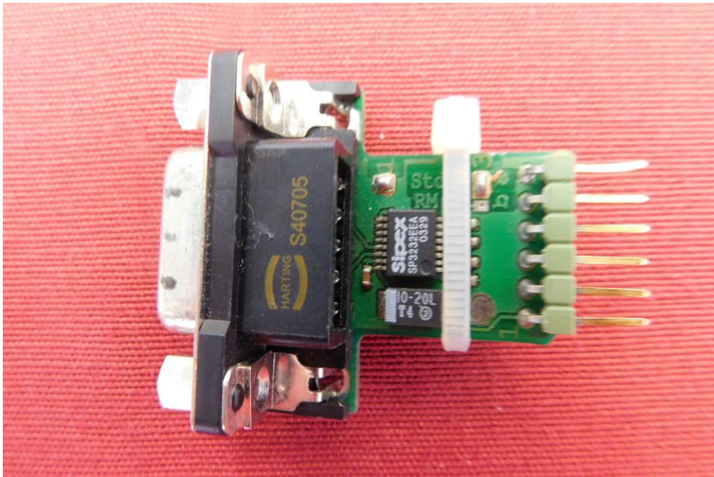
Picture 17: Top view of RS232 connector
