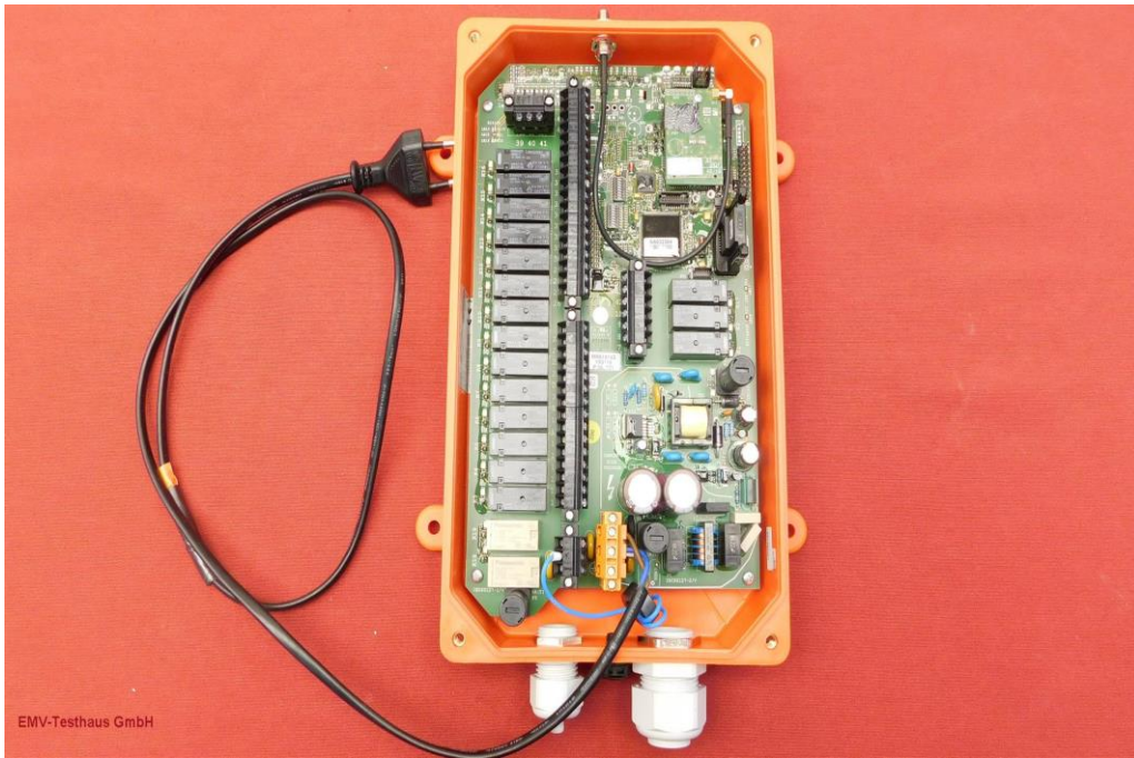
Picture 15: Top view of opened companion device
