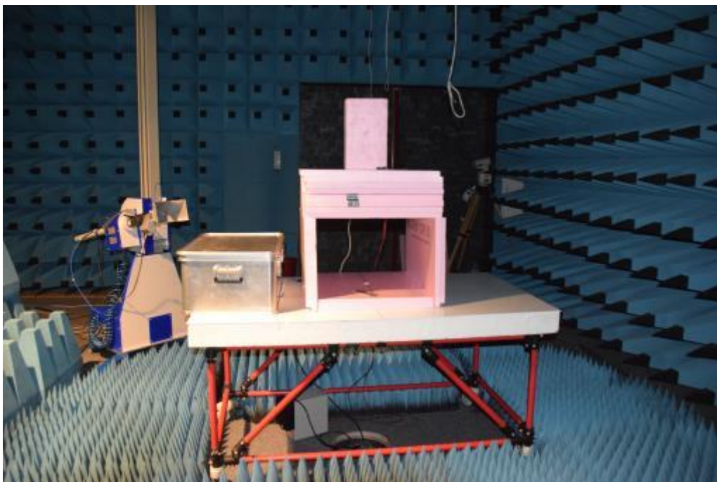
Picture 8: AC, radiated emission test 1 GHz – 17 GHz – position Y (back view)
