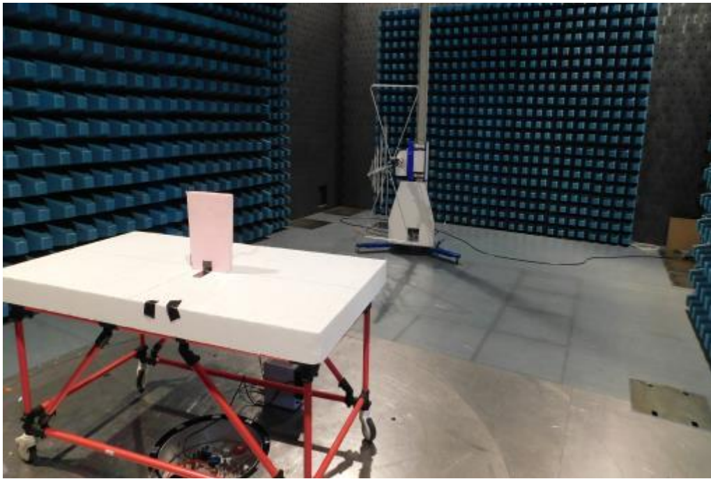
Picture 5: SAC, radiated emission test 30 MHz – 1 GHz – position Y (front view)
