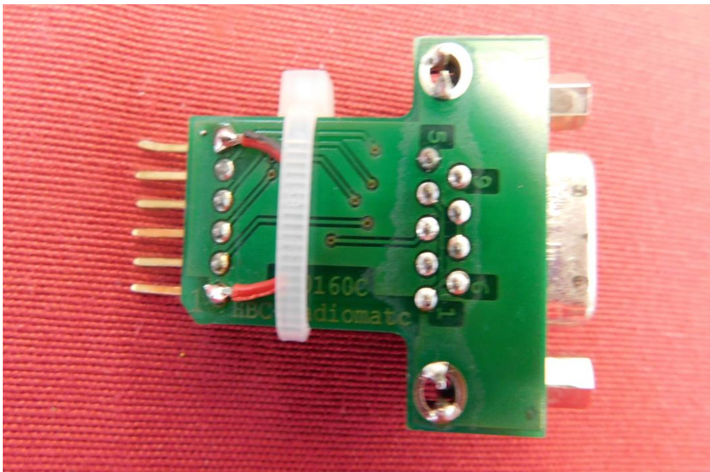
Picture 18: Back view of RS232 connector
