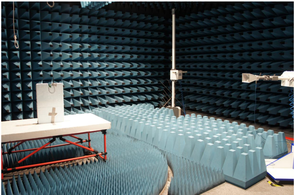
Picture 6: EUT test setup radiated emission test 1GHz – 26GHz
