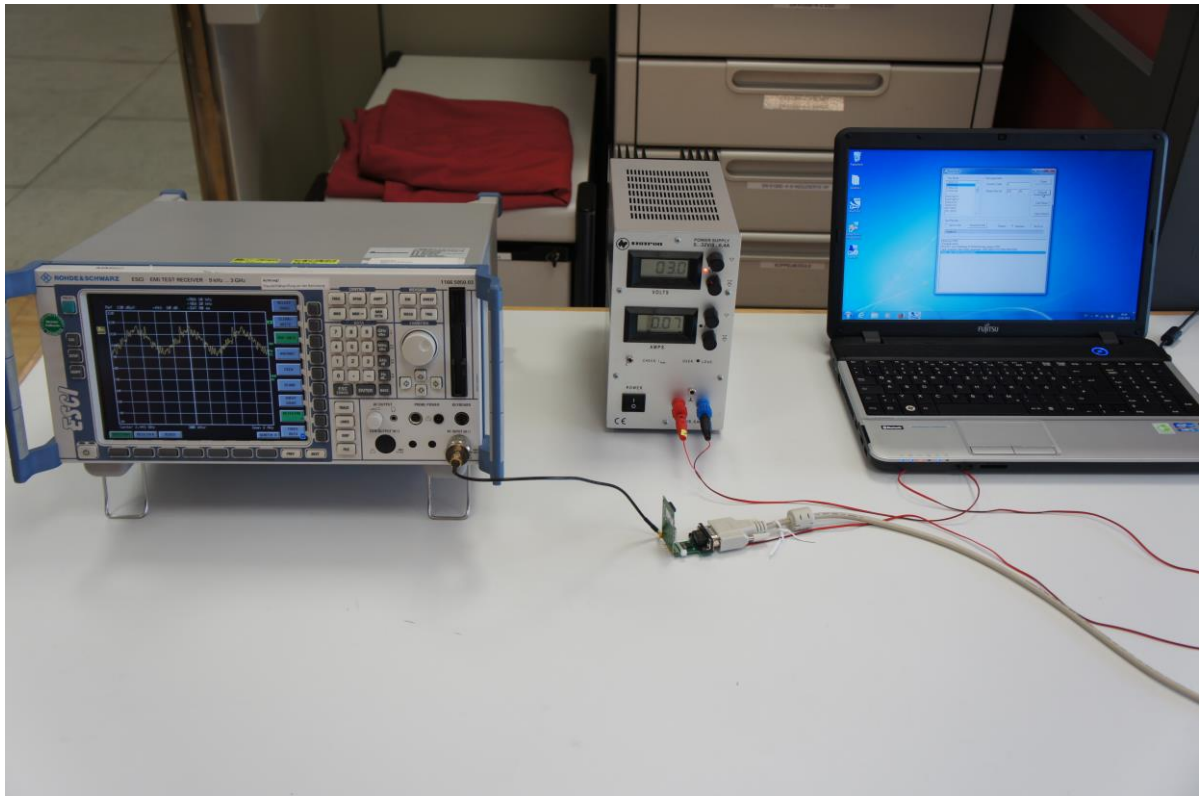
Picture 3: EUT test setup conducted measurements
