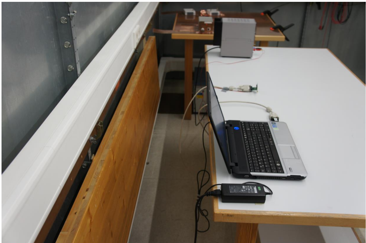
Picture 2: EUT test setup AC power line conducted emissions (rear view)
