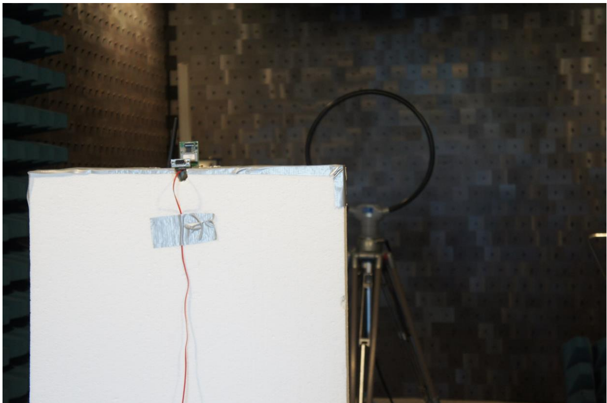
Picture 4: EUT test setup radiated emission test 9 kHz - 30 MHz
