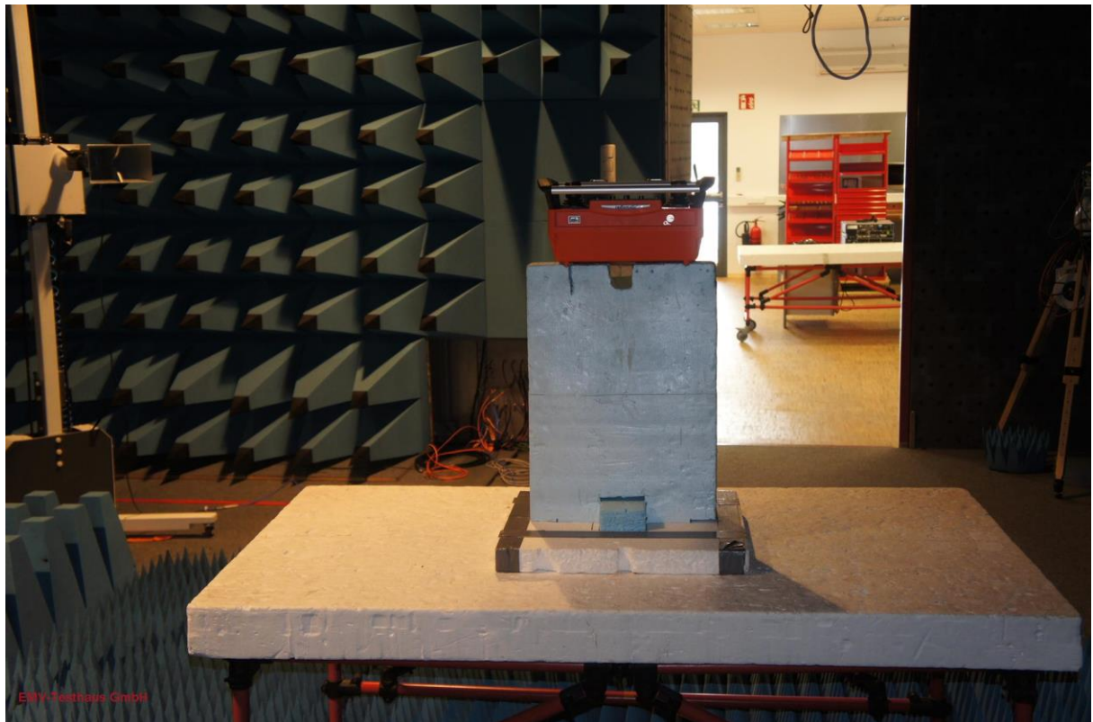
Picture 7: AC, test setup radiated emission test > 1 GHz (rear view)
