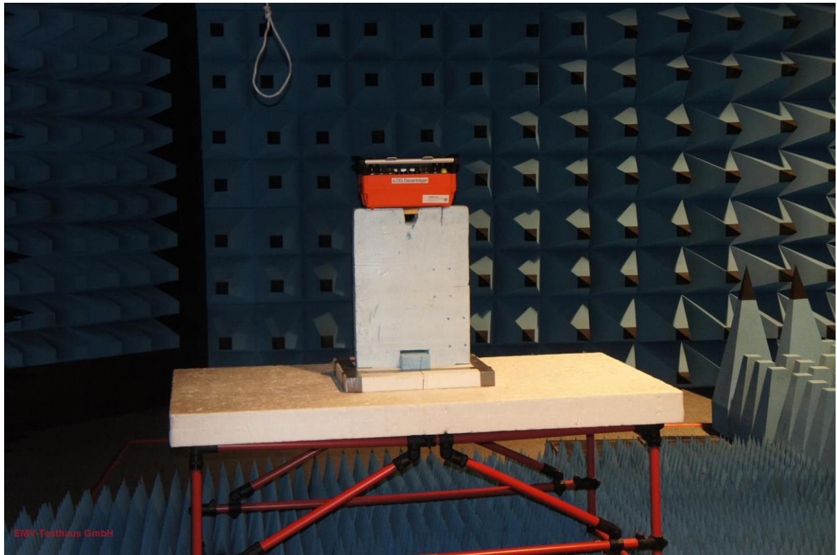
Picture 6: AC, test setup radiated emission test > 1 GHz (front view)
