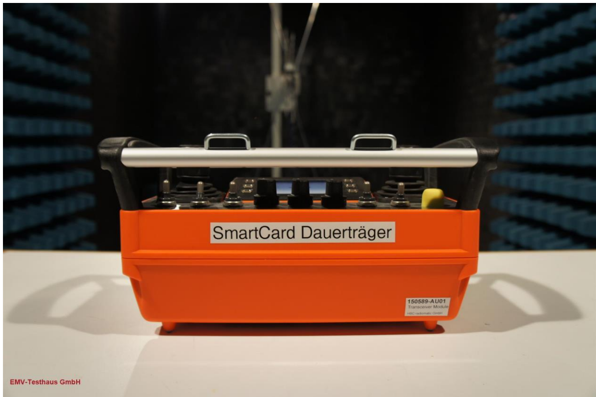
Picture 9: EUT-position 1
