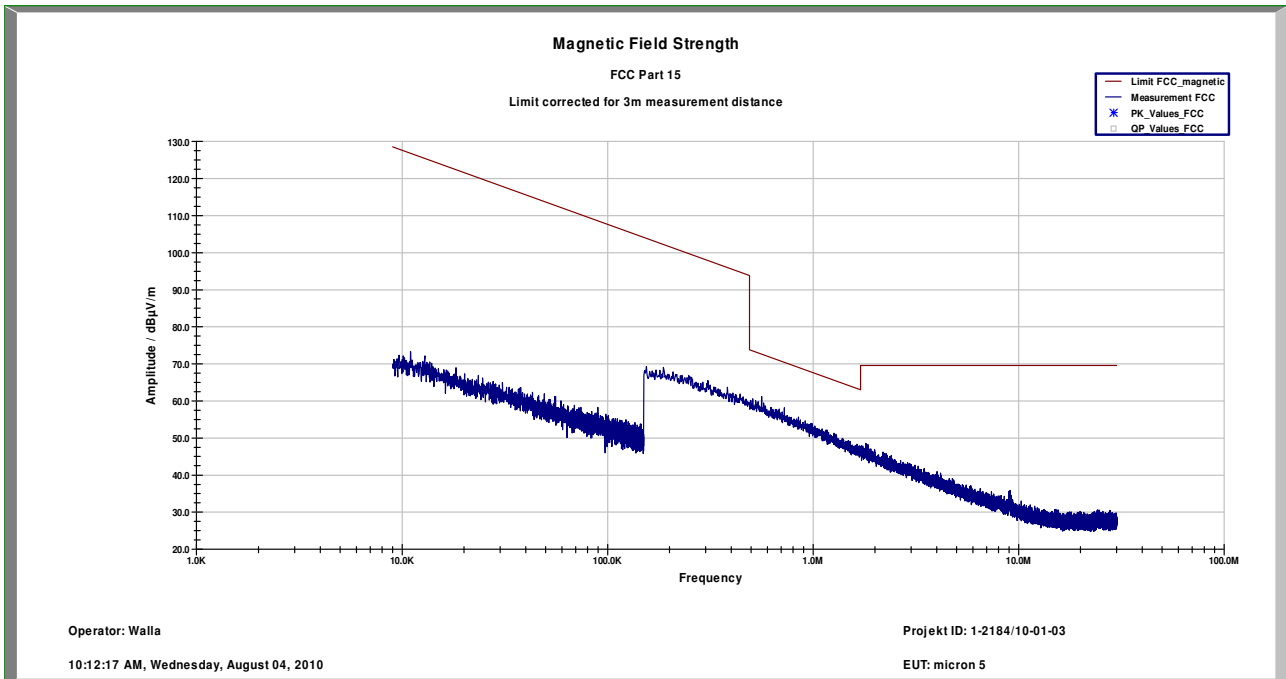
Plot 2: RX-Mode, 9 kHz – 30 MHz @ 3 m
