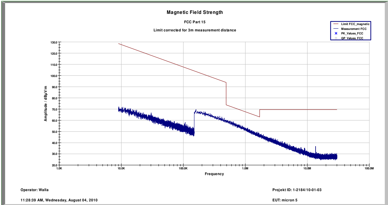
Plot 1: TX-Mode, 9 kHz – 30 MHz @ 3 m
