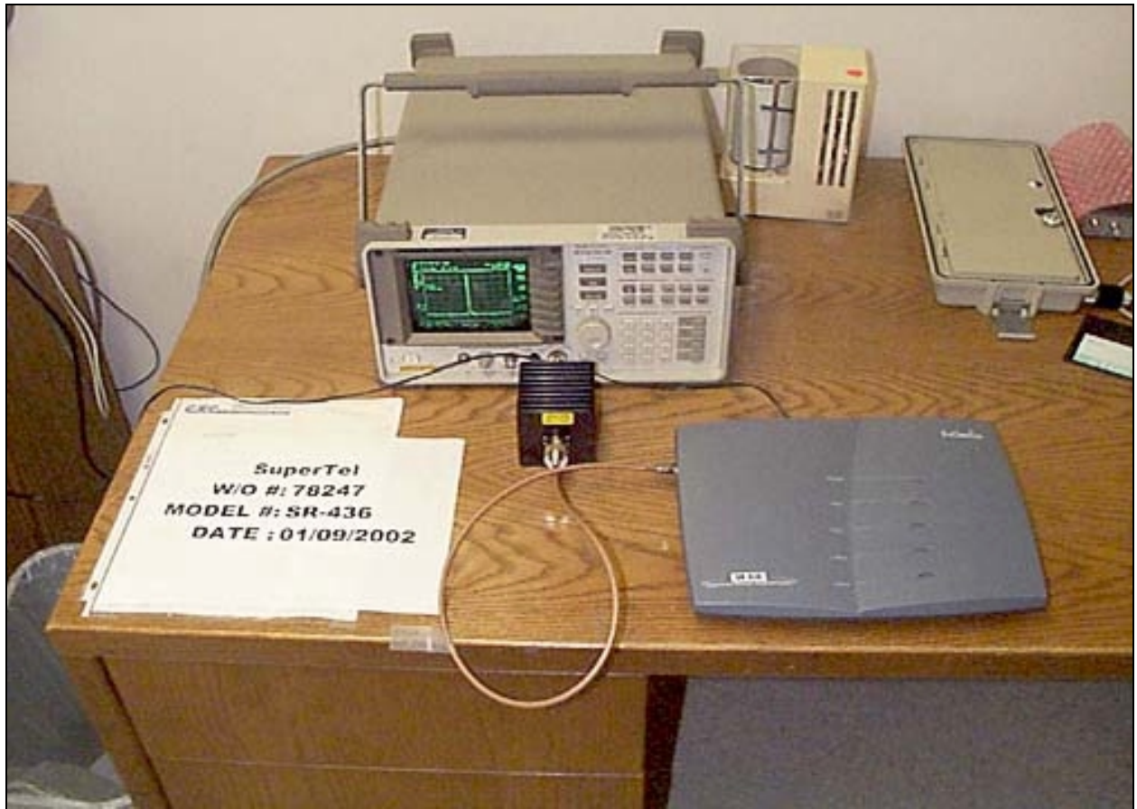
PHOTOGRAPH SHOWING ANTENNA CONDUCTED EMISSIONS - BASE
