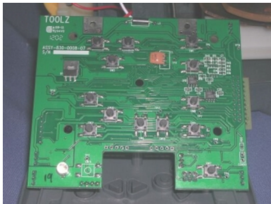
Internal Photo - 12
