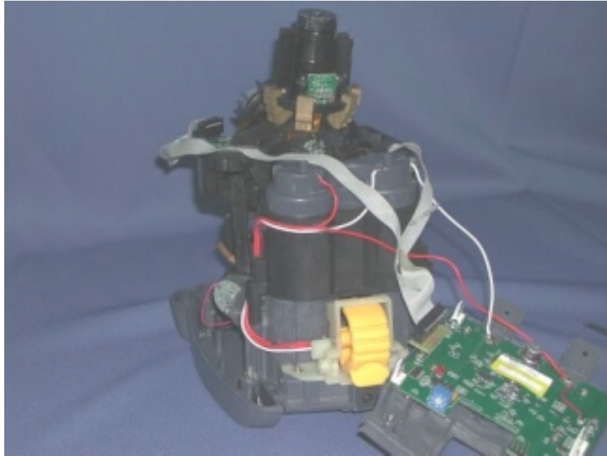
Internal Photo - 13
