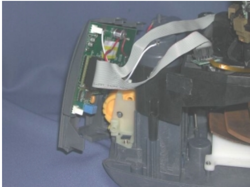
Internal Photo - 10
