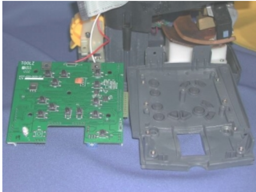
Internal Photo - 12
