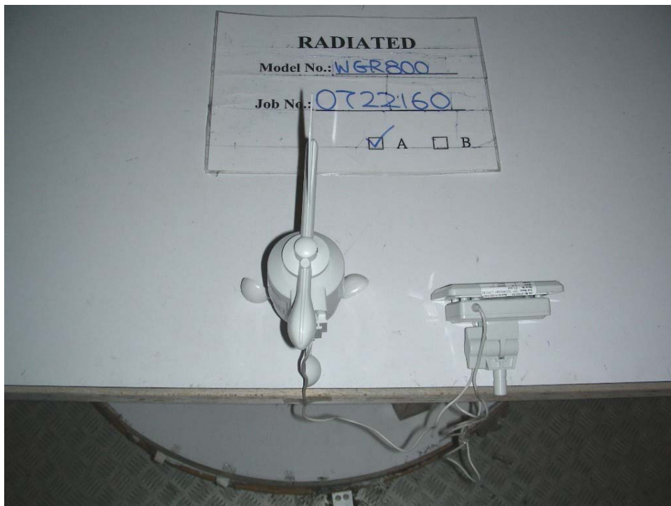
Radiated - rear
