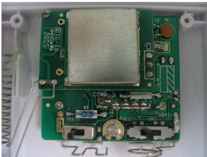
Transmitter
