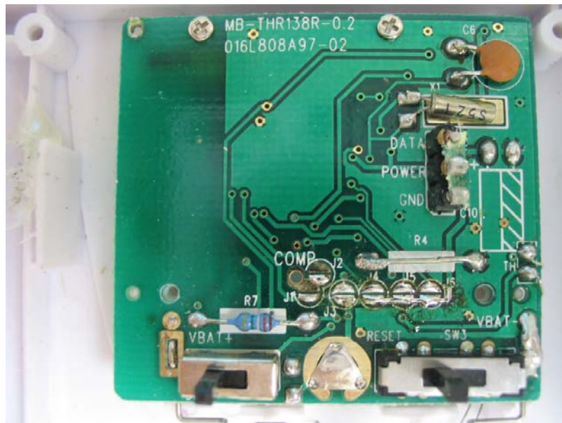
Transmitter
