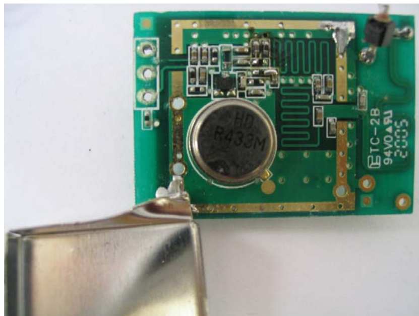
Transmitter
