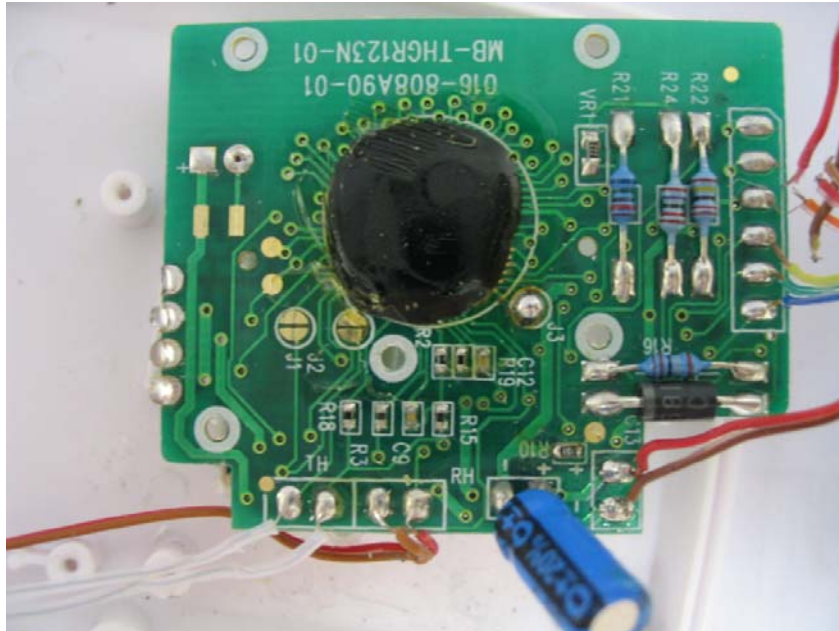
Transmitter
