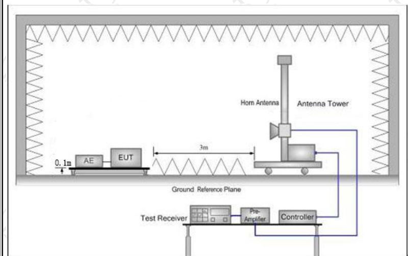
Above 1GHz
