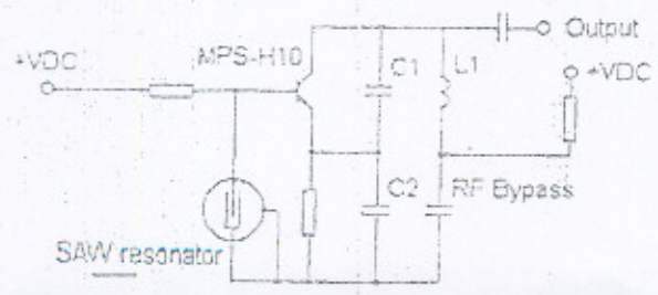
Typical Local Oscillator Application
