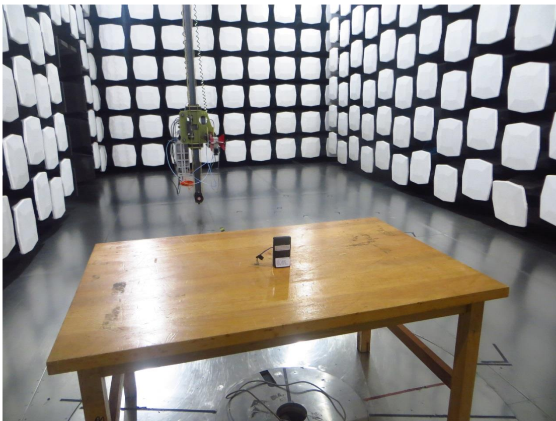
Above 1 GHz
