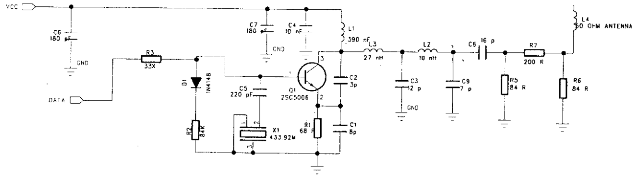
UHF TRANSMITTER
