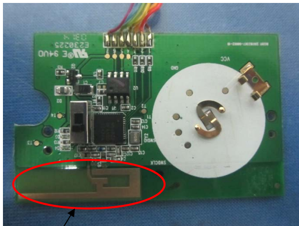
RF Antenna
