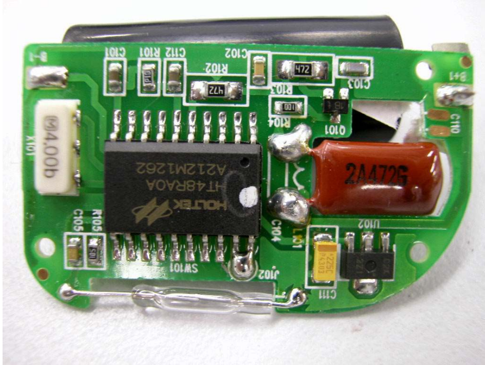
Internal Photo – 2 (Speed Sensor)
