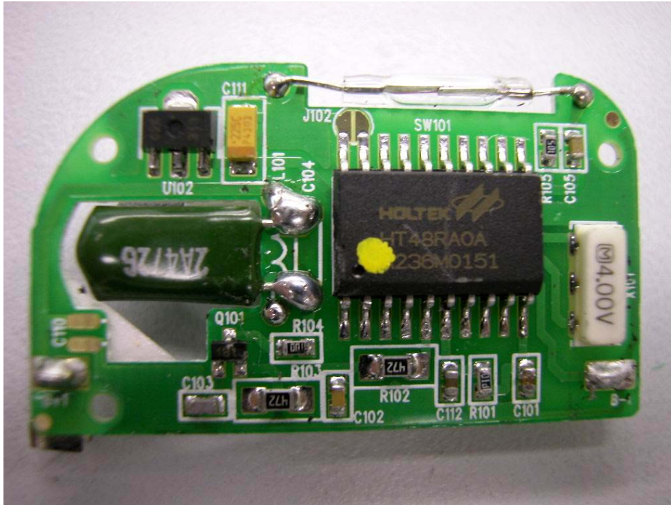
Internal Photo – 2 (Cadence Sensor)
