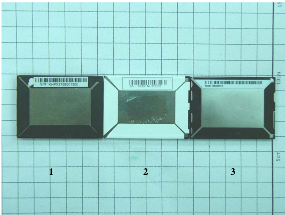
Fig.28 Back view of Battery: 1. Simplo, 2.samsung, 3.sanyo
