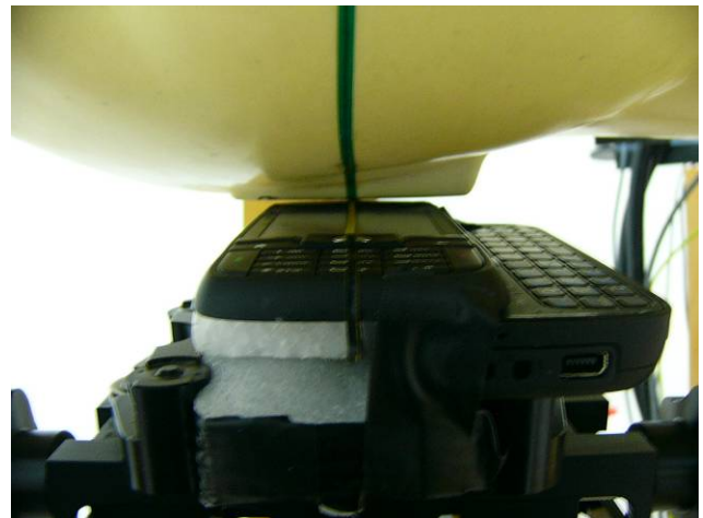
Fig.10 Left Head at Slider-on Section / Ear-Tilt Position(15°)
