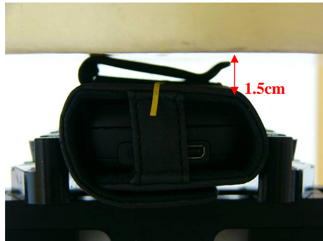
Fig.12 Body worn with Holster 1- EUT back to flat phantom (testing in GPRS Mode), distance between flat phantom and mobile phone is 1.5 cm
