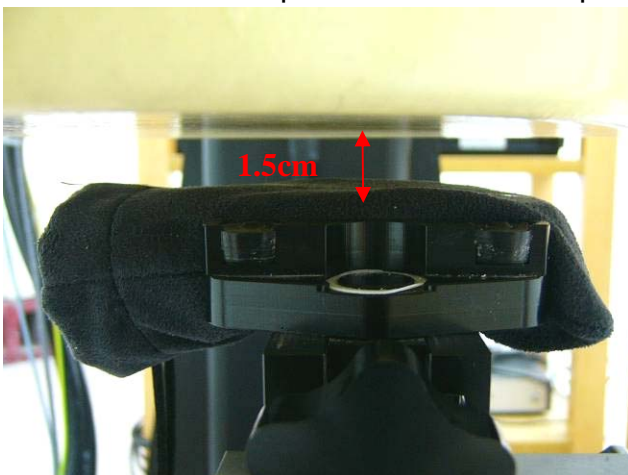
Fig.13 Body worn with Holster2- EUT front to flat phantom (testing in GPRS Mode), distance between flat phantom and mobile phone is 1.5 cm
