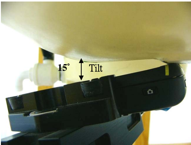
Fig.6 Left Head at Slider-off Section / Ear-Tilt Position(15°)
