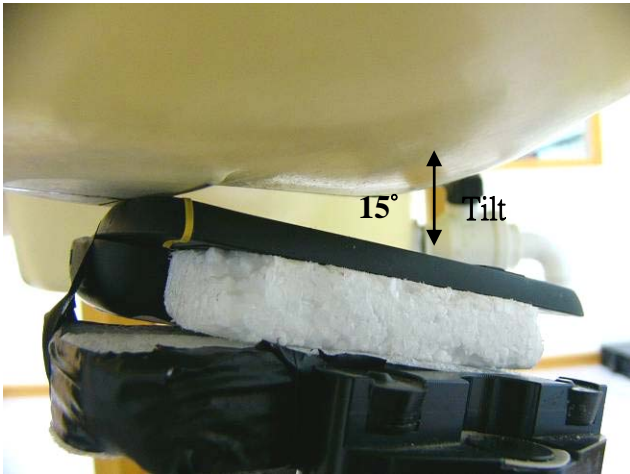
Fig.8 Right Head at Slider-on Section / Ear-Tilt Position(15°)
