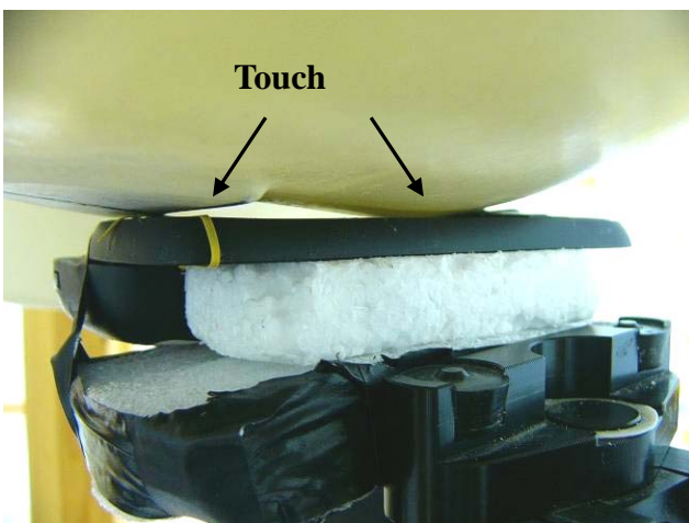
Fig.7 Right Head at Slider-on Section / Cheek-Touch Position
