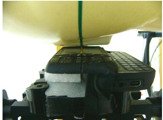
Fig.8 Right Head at Slider-on Section / Ear-Tilt Position(15°)
