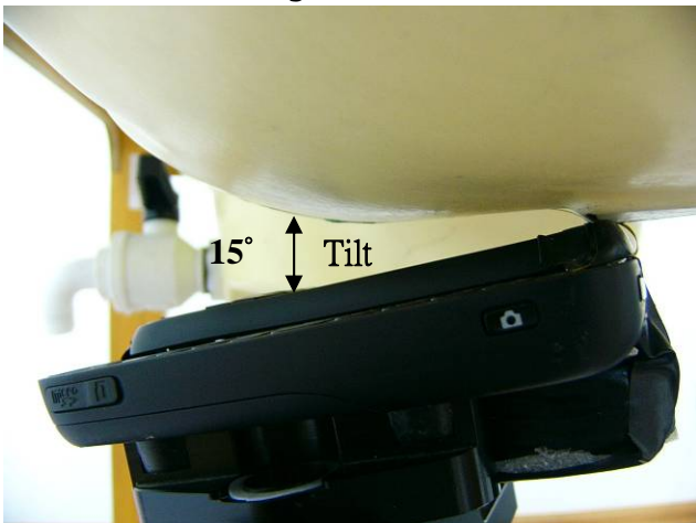
Fig.10 Left Head at Slider-on Section / Ear-Tilt Position(15°)
