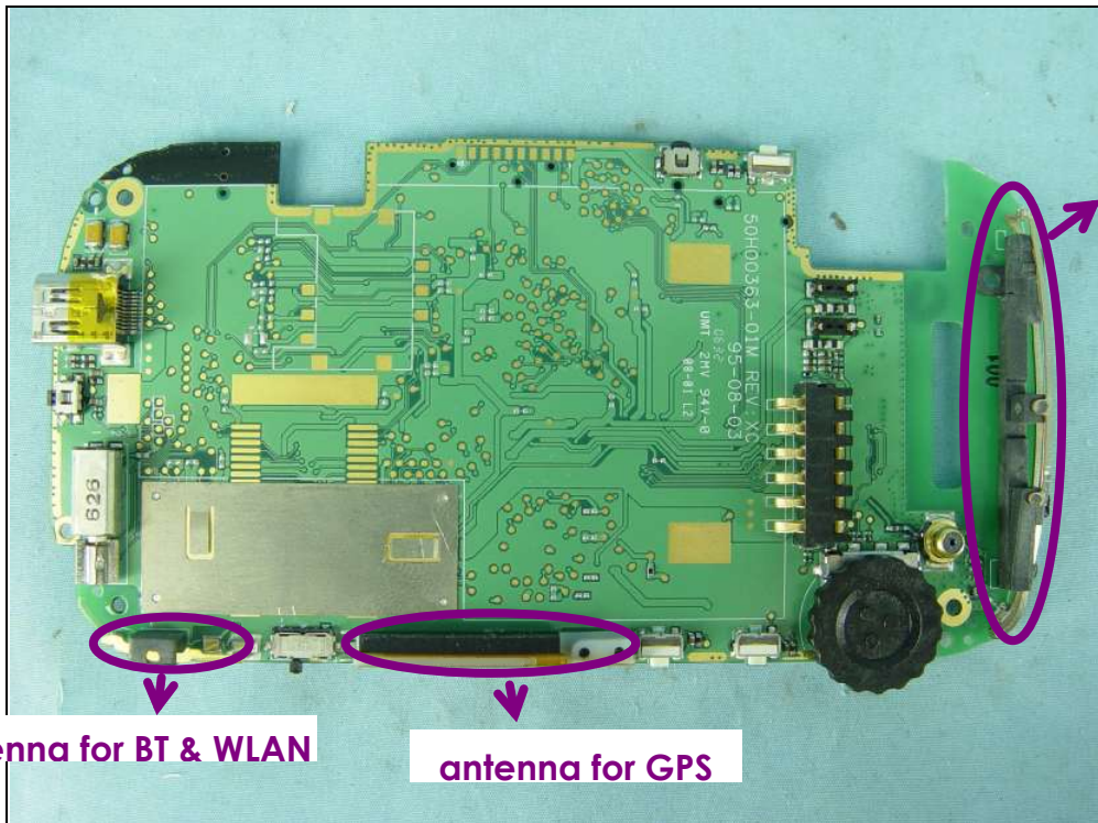
antenna for CDMA
