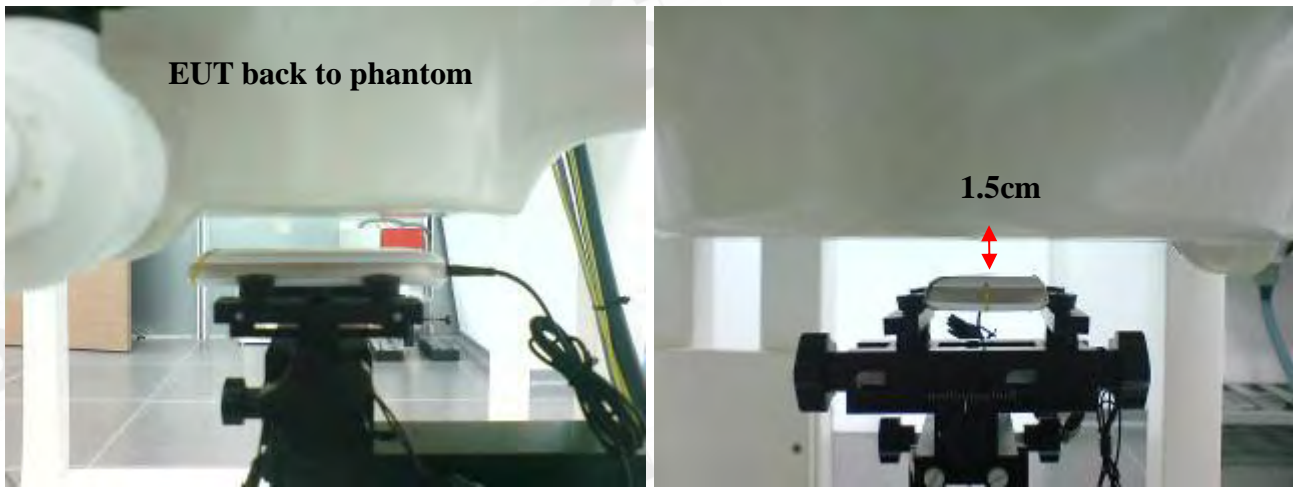
Fig.8 Body worn- EUT back to flat phantom and distance between flat phantom and mobile phone is 1.5 cm with headset
