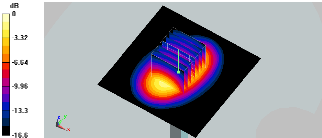
0 dB = 4.8mW/g
