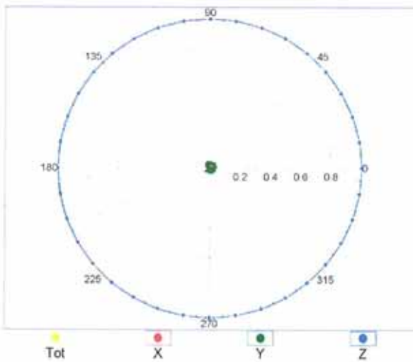
f=600 MHz,TEM,90°
