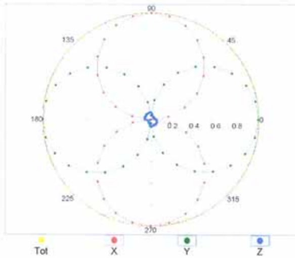
f=600 MHz,TEM,0°
