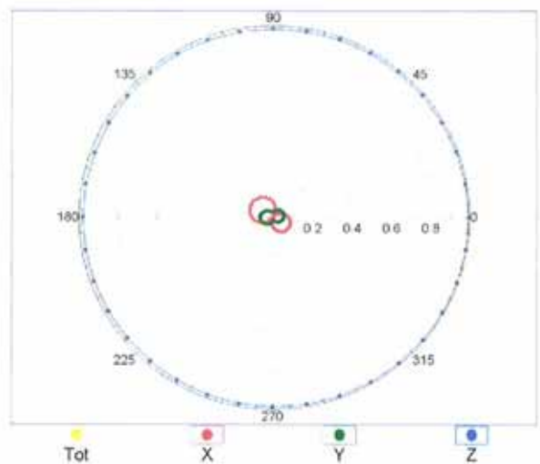
f=2500 MHz,R22,90°
